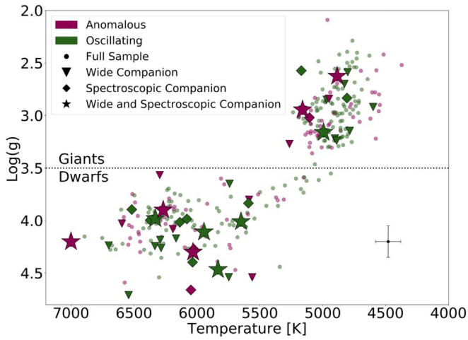
Figure 7. H–R diagram showing the full sample of oscillating (green) and anomalous (purple) stars with surface gravity on the y-axis and temperature on the x-axis (both from KSPC). The error shown (100 K for temperature and 0.15 dex for surface gravity) is a typical uncertainty for the whole sample. A line separates the dwarfs and giants at \log(g) = 3.5 . The circles in this plot represent the targets for which no companions were found. Targets with a wide companion are shown by a downward facing triangle, the spectroscopic binaries are marked by a diamond and targets with both a wide and spectroscopic companion are marked by a star.
