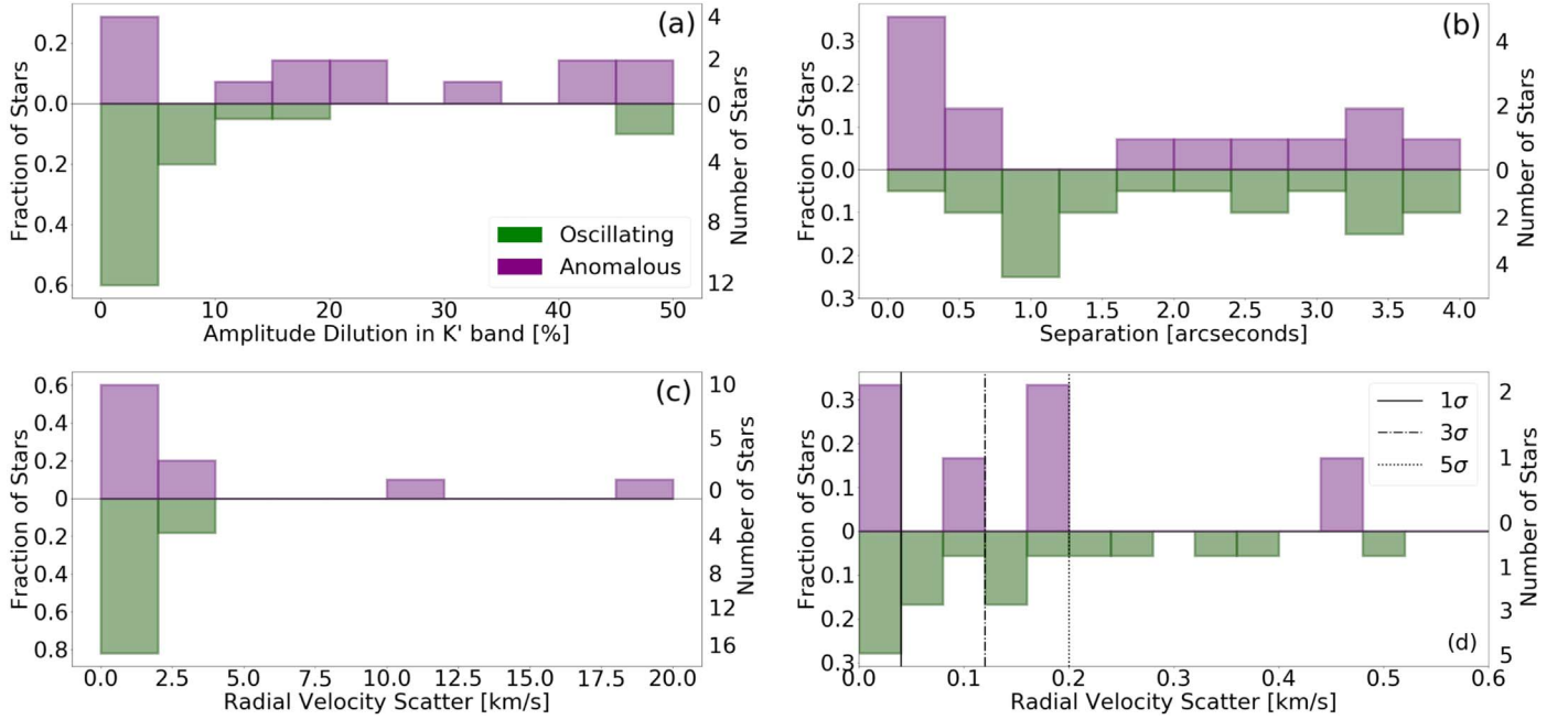
Figure 9. Plots showing the distribution of companion systems in the oscillating and anomalous groups as a function of system parameters. Top left: distribution as a function of amplitude dilution in the K' -band (%). Top right: distribution as a function of separation from the primary star (arcseconds). Bottom left: distribution as a function of the radial velocity scatter ( \text{km s}^{-1} ). Bottom right: distribution as a function of radial velocity scatter up to 0.6 \text{ km s}^{-1} ( \text{km s}^{-1} ). Also showing 1\sigma , 3\sigma , and 5\sigma lines.
