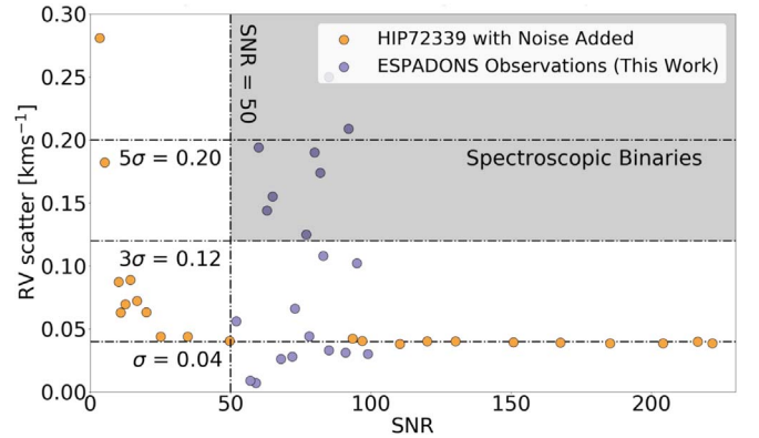
Figure 6. Radial velocity scatter vs. S/N. Orange symbols represent the standard star with a varying S/N, simulated by adding Gaussian noise to the spectra. Purple symbols illustrate our target sample. The horizontal dashed line marks the 1\sigma limit. Above 3\sigma we define our targets to be RV variable due to a stellar companion (shaded area). The y-axis has been truncated to not include the larger values of RV scatter.
