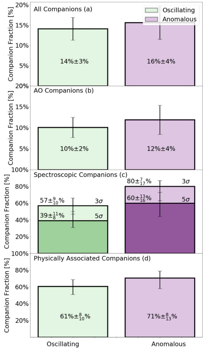
Figure 8. Companion fractions for oscillating (green) and anomalous (purple) systems. Top: all companion systems. Second from top: AO/wide companions. Third from top: spectroscopic companions. Bottom: physically associated companions. Uncertainties are calculated using binomial or Poisson statistics depending on the sample size.
