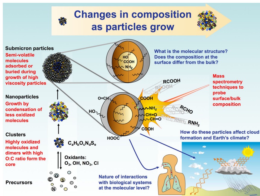
Fig. 1 Schematic of the life cycle of secondary organic aerosol particles and their impacts. Volatile organic precursors are oxidized in air by O_3 , OH , NO_3 , or Cl , and the resulting highly oxygenated, low-volatility products formed from these reactions nucleate new particles, and/or condense on pre-existing ones to grow them. Different species participate in particle growth at different stages of the life cycle, with less oxygenated, more volatile species condensing on the larger particles. Chemical composition of these SOA particles will depend on the environmental conditions surrounding the particles (relative humidity, temperature, gas phase composition ...etc.), as well as their physical properties (i.e., viscosity) governing the uptake of trace gases. Once they reach \sim 50 – 100 nm, these particles are able to impact climate directly by interacting with incoming solar radiation but also indirectly via cloud processing. The chemical composition and size of these particles will also determine their impact on health.
