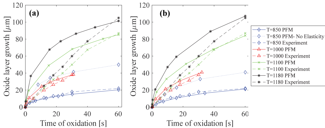
Figure 1. Oxide layer growth at different temperatures (°C) for a diffusive interface thickness of (a) \lambda = 40\text{ nm} and (b) \lambda = 800\text{ nm} . Experimental results are obtained from [31].
