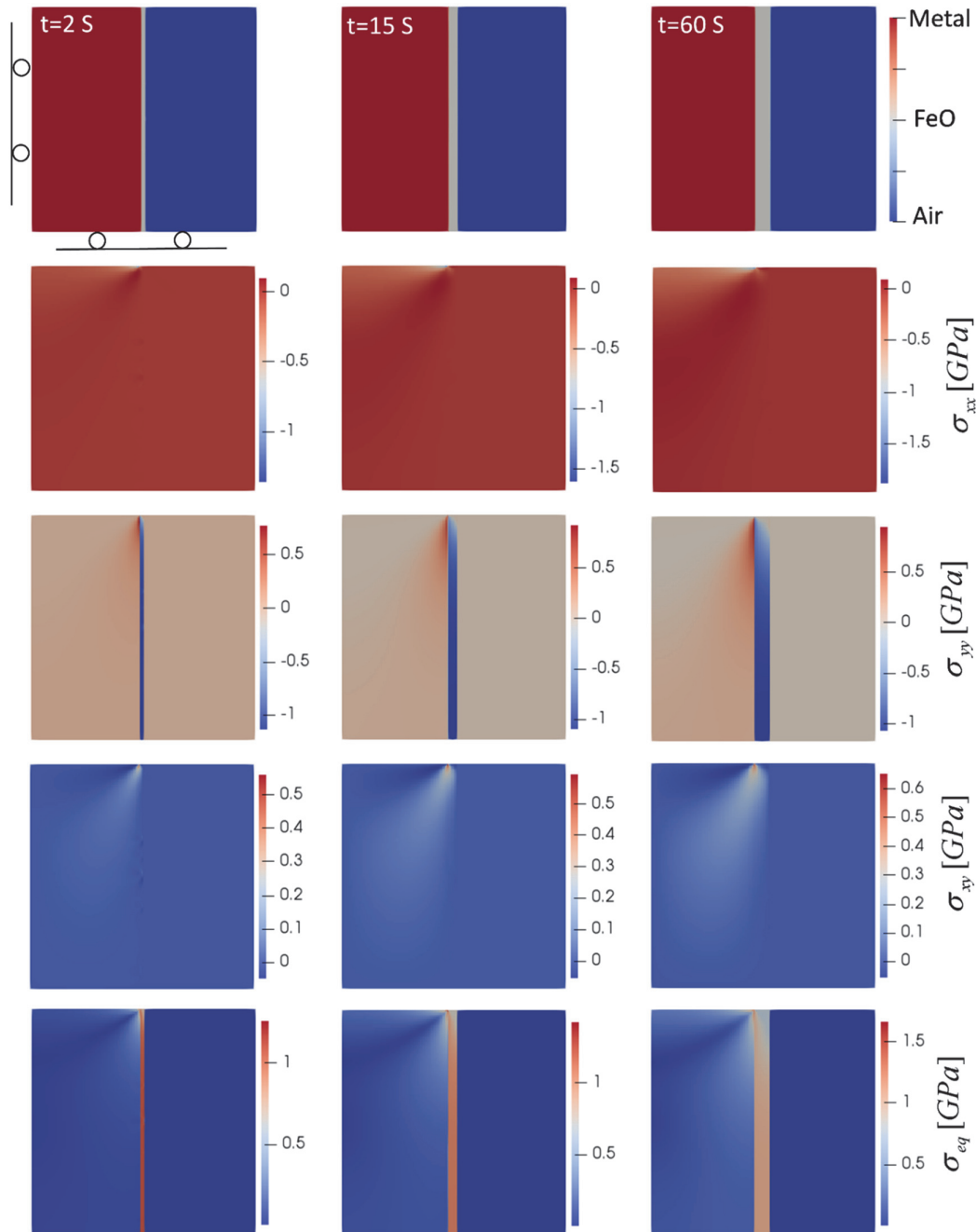
Figure 3. Oxide layer growth and evolution of induced stresses in planar oxidation ( T = 850\text{ }^{\circ}\text{C} ). Domain size is 0.5\text{ mm} \times 0.5\text{ mm} . Top left snapshot also shows the mechanical boundary conditions.
