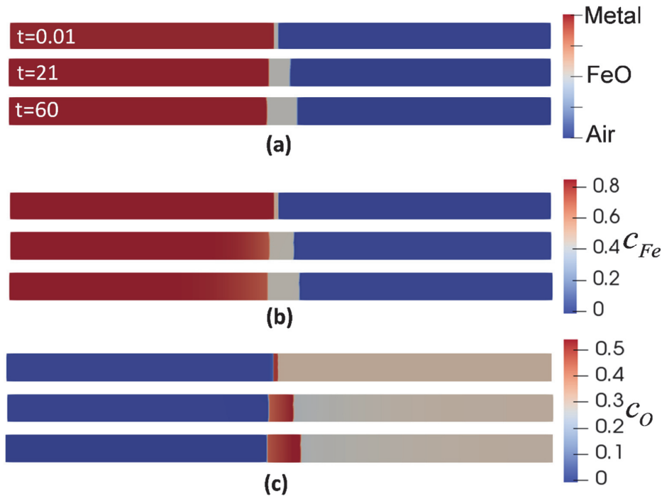
Figure 2. Evolution of phase-field (PF) variables during oxidation at temperature of 850\text{ }^{\circ}\text{C} . (a) phases (b) concentration of Iron (c) concentration of oxygen.
