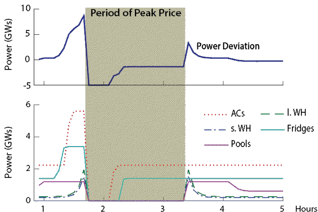
Figure 2. The optimal response of millions of air conditioners, water heaters, refrigerators and pool pumps to a 90-minute increase in electricity price, given quality of service guarantees (Cammardella, 2018). The resulting fast load ramps could become a major headache for grid operators, and many loads are not able to hold their response through long events.
