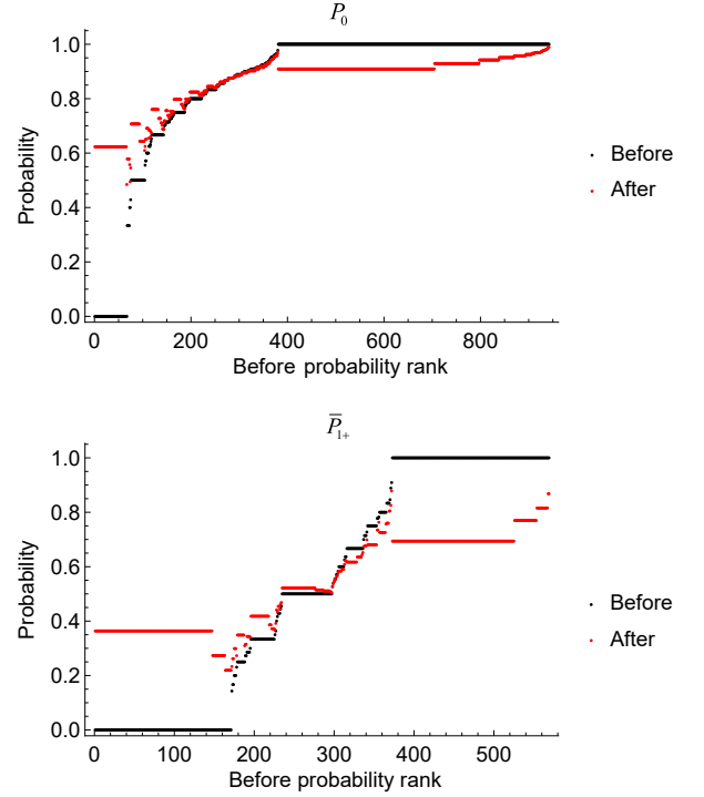
Fig. 7. Stopping probabilities before and after Bayesian updating
