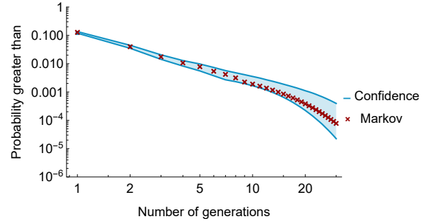
Fig. 4. Survival function of cascade sizes. Red crosses are from Markov chain, and blue lines indicate the 95% confidence interval estimated by bootstrap.
