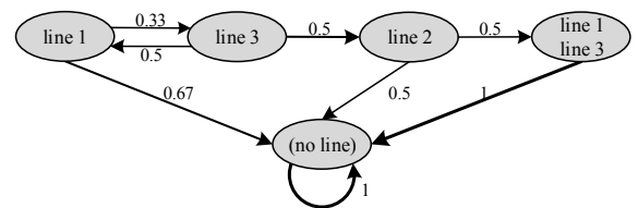
Fig. 1. Simple example forming influence graph from artificial data (real utility data is shown in Fig. 2).
