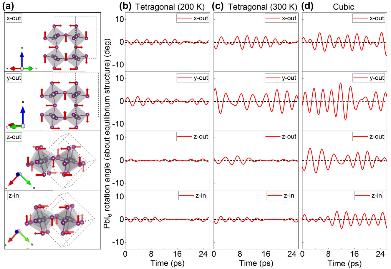
FIG. 3. Contrasting the \text{PbI}_6 rotational motions in the t and c phases. (a) Illustrations of real-space \text{PbI}_6 rotational motions. (b)–(d) Time evolution of \text{PbI}_6 rotation amplitudes in the t phase at (b) 200 K, (c) 300 K, and (d) the c phase. The legend reports the rotation axis and the relative rotation direction. For example, x -out represents the out-of-phase rotation along the x axis, and z -in represents the in-phase rotation along the z axis. These amplitudes are obtained from MD trajectories frequency-filtered to 1 \text{ cm}^{-1} . The black dashed lines at 0^\circ represent the equilibrium tilting angle of the octahedra around each axis, which has been offset to the 0^\circ for a clearer comparison. The equilibrium angle can be found in Table S2.
