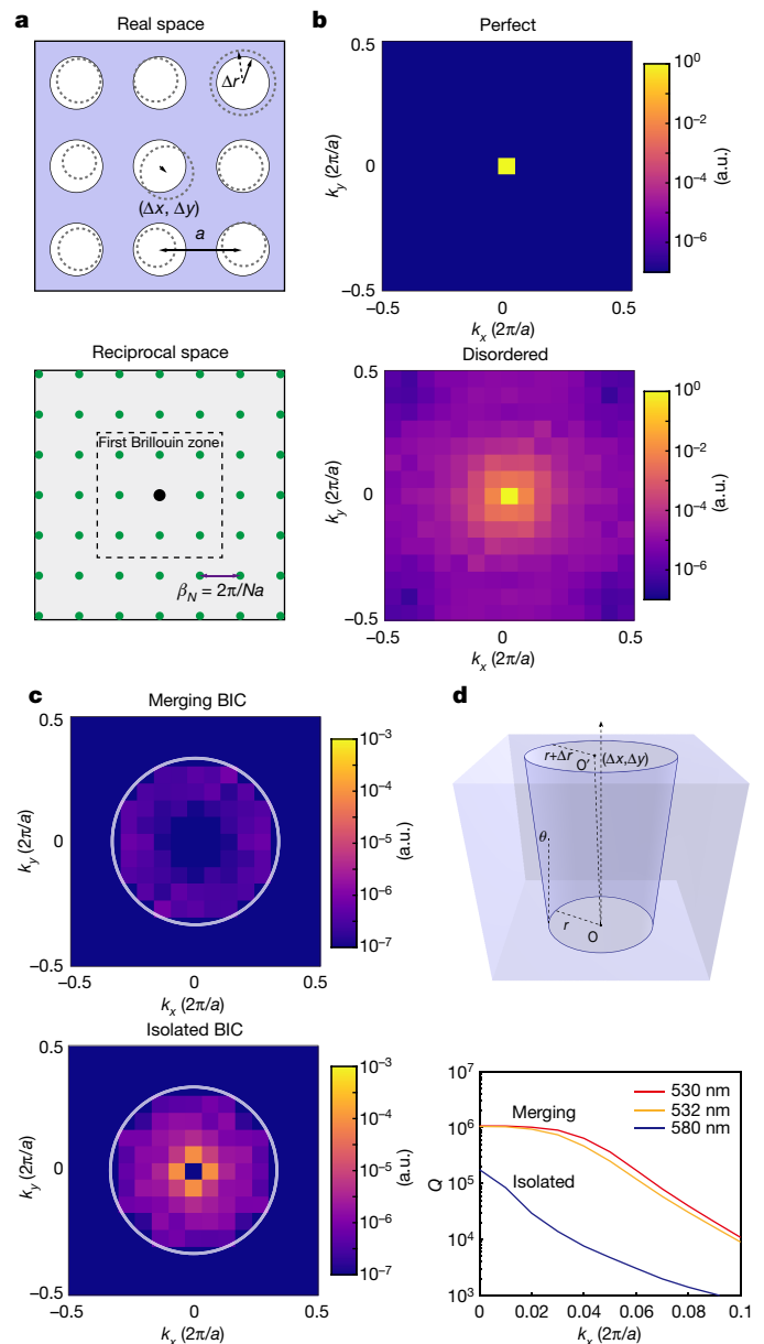
Fig. 2 | Topological protection against scattering losses. a , Schematic of a fabricated photonic crystal sample (solid lines; top), with disorder in the locations and radii of the holes (dashed lines; top). In reciprocal space, fractional orders of momentum (green dots; bottom) are introduced by the supercell. N is the size of the supercell in increments of the periodicity a and \beta_N is the minimum step size of the fractional orders of momentum. b , Momentum-energy distribution of the highest- Q mode in the merging-BIC design for a perfect (top) and a disordered (bottom) structure inside the first Brillouin zone. a.u., arbitrary units. c , Momentum-energy distribution of the radiation field in the disordered merging-BIC (top) and isolated-BIC (bottom) designs. The white circles represent the light cone—the region in the momentum space where guided resonance can couple to the radiation channel, as determined by the structure of the sample. The scattering loss is considerably lower in the merging-BIC sample than in the isolated-BIC sample. d , Schematic of an asymmetric hole (top) acting as a fabrication imperfection, and simulated Q values near the centre of the Brillouin zone obtained by the application of disorder (bottom). All simulations were performed in a 15a \times 15a supercell ( N = 15 ).
