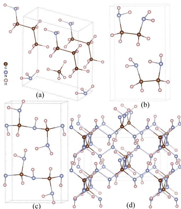
Figure 2 Crystal structures of \text{CH}_4\text{-N}_2 compounds. (a) P1 phase at 10 GPa for \text{C}_2\text{NH}_8 . This phase can be seen as a mixture of molecular units: \text{C}_3\text{NH}_9 + \text{NH}_3 + \text{CH}_4 . (b) P2_1 structure for \text{CNH}_4 at 50 GPa. This phase can be seen as a molecular phase with formula units \text{C}_2\text{N}_2\text{H}_8 . (c) the polymeric Pca2_1 phase of \text{CN}_2\text{H}_4 at 20 GPa. (d) I-42d phase of \text{CN}_4\text{H}_4 at 50 GPa.
