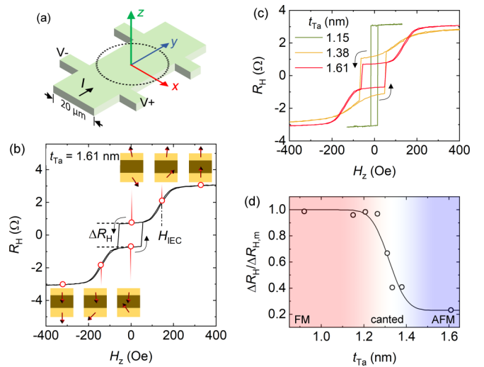
FIG. 3. (a) The schematic of the Hall bar structure. (b) Hall resistance R_H vs perpendicular magnetic field H_z for a magnetic-multilayer structure with t_{\text{Ta}} = 1.61 \text{ nm} and t_{\text{CoFeB}} = 1.12 \text{ nm} . The inserts show schematics of magnetic configurations at different perpendicular magnetic fields. \Delta R_H is the difference between Hall resistances for two opposite spin states at zero magnetic field. (c) Hall resistance R_H vs perpendicular magnetic field H_z for magnetic multilayers with different t_{\text{Ta}} and with the same ferromagnetic layer thickness of t_{\text{CoFeB}} = 1.12 \text{ nm} . (d), \Delta R_H/\Delta R_{H,m} as a function of t_{\text{Ta}} . Dots are experimental data and the line is a guide for the eyes. Arrows in (b) and (c) represent switching directions.
