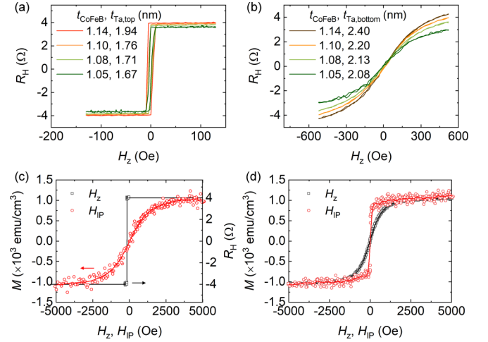
FIG. 2. (a) Hall resistance measurement for the structure of \text{Ta}(t_{\text{Ta,top}})/\text{Co}_{40}\text{Fe}_{40}\text{B}_{20}(0.8t_{\text{CoFeB}})/\text{MgO}(1.6)/\text{TaO}_x(2.0) (top structure). The results were measured through Hall bars located at different positions on the sample with different \text{Ta}(t_{\text{Ta,top}}) and \text{Co}_{40}\text{Fe}_{40}\text{B}_{20}(0.8t_{\text{CoFeB}}) layer thicknesses. (b) Hall resistance measurement for the structure of \text{MgO}(1.6)/\text{Co}_{40}\text{Fe}_{40}\text{B}_{20}(t_{\text{CoFeB}})/\text{Ta}(t_{\text{Ta,bottom}}) (bottom structure). The results were measured through Hall bars located at different positions on the sample with different \text{Ta}(t_{\text{Ta,bottom}}) and \text{Co}_{40}\text{Fe}_{40}\text{B}_{20}(t_{\text{CoFeB}}) layer thicknesses. (c) The magnetization measurement (red circle dots) and the Hall resistance measurement (black square dots) with applications of the in-plane magnetic field H_{\text{IP}} and the perpendicular magnetic field H_z , respectively, for the top structure. (d) The magnetization measurement with applications of the in-plane magnetic field H_{\text{IP}} (red circle dots) and the perpendicular field H_z (black square dots), for the bottom structure. In (c) and (d), dots are experimental results and lines are to guide the eye.
