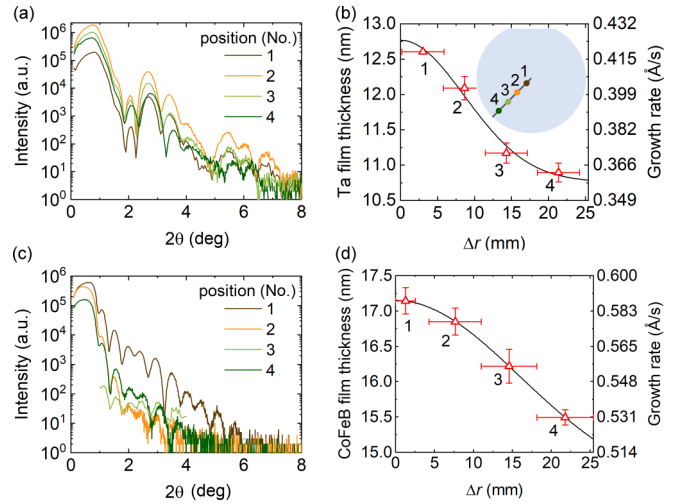
FIG. 1. (a) X-ray reflection measurements at four different positions of a Ta film that was deposited in 300.9 s. Four illumination positions are schematically presented in the inset in (b). (b) Ta film thicknesses and growth rates at different radial positions, obtained from x-ray reflection measurements. \Delta r is the radial distance between the illumination point and the center of the silicon wafer. (c) X-ray reflection measurements at four different positions of a Co 40 Fe 40 B 20 film that was deposited in 291.8 s. (d) Co 40 Fe 40 B 20 film thicknesses and growth rates at different radial positions, obtained from x-ray reflection measurements. Error bars were derived from the measurements and uncertainty of illumination positions.
