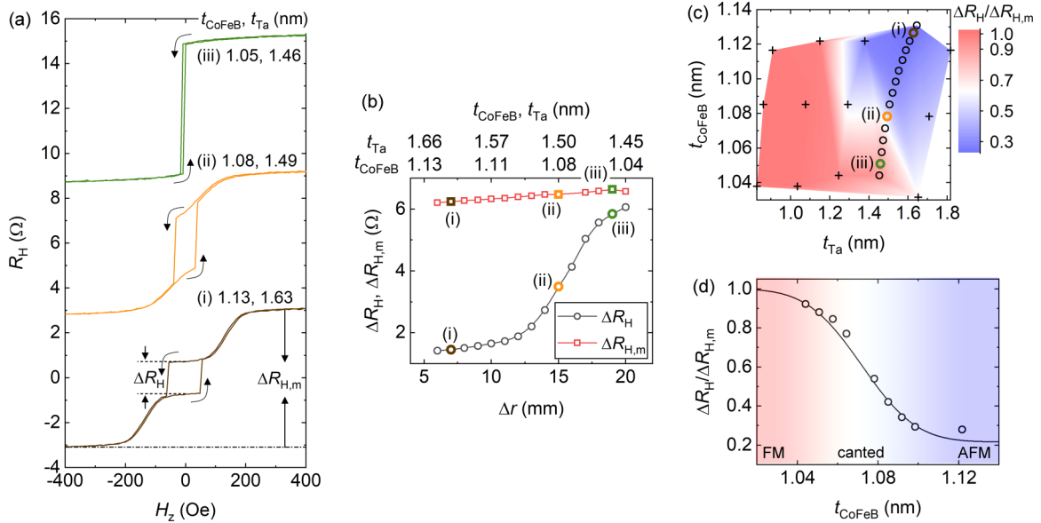
FIG. 4. (a) Hall resistance R_H vs perpendicular magnetic field H_z for Hall bars at different positions in a single batch. \Delta R_{H,m} is the difference between Hall resistances for two opposite spin states at positive and negative saturation fields. (b) \Delta R_H and \Delta R_{H,m} as a function of the radial distance \Delta r in a single batch. The data correspond to the array of circles in (c). In (b), labels of t_{Ta} and t_{CoFeB} are also given. (c) Phase diagram of \Delta R_H/\Delta R_{H,m} as functions of both Ta spacer thickness t_{Ta} and the \text{Co}_{40}\text{Fe}_{40}\text{B}_{20} layer thickness t_{CoFeB} . Crosses and circles indicate corresponding t_{Ta} and t_{CoFeB} of magnetic multilayers at different positions where Hall bars locate. Circles correspond to the data in (b). The blue area refers to the antiparallel magnetization of the ferromagnetic layers, and the red area refers to the parallel magnetization of the ferromagnetic layers. The area with light colors refers to the canted magnetization state. (d) \Delta R_H/\Delta R_{H,m} as a function of t_{CoFeB} . The data are collected for samples with t_{Ta} in the 1.3–1.55-nm range. Arrows in (a) represent switching directions.
