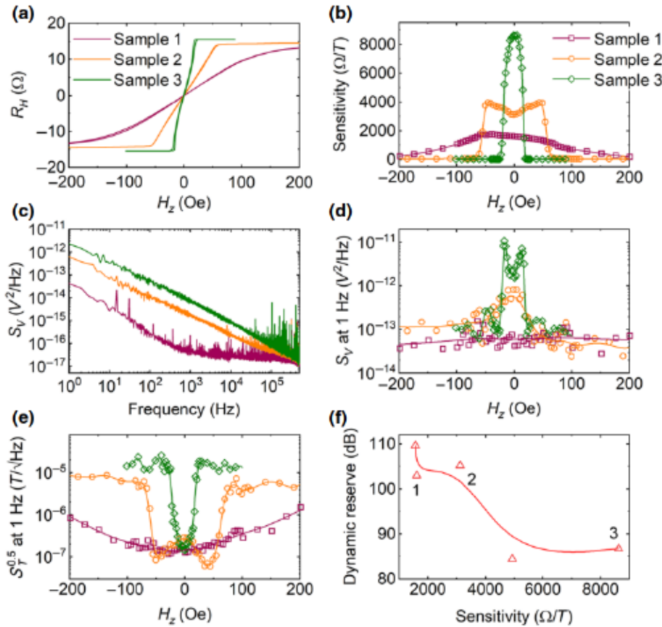
FIG. 3. (a) Anomalous Hall loops of three magnetic multilayers with different perpendicular anisotropies. Sample 1 has the magnetic layer thickness t_1 = 0.8 nm ( t_2 = 1.0 nm), while sample 2 and sample 3 have the magnetic layer thicknesses t_1 = t_2 = 0.9 nm. (b) The anomalous Hall sensitivity measured at different perpendicular magnetic field H_z . (c) Noise spectra for three samples measured at zero magnetic field. (d) The intrinsic noise, and (e) magnetic field detectability at 1 Hz as a function of H_z . (f) The dynamic reserve for three samples and the other two samples with similar structures.
