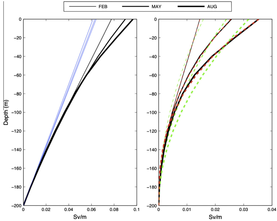
Fig. 2.7. (Left) Typical transport profile anomaly relative to 200 dbar for February, May and August on the western boundary. Blue lines indicate linear extrapolation from 200 dbar. (Right) Black lines indicate the residual dynamic height anomaly after linearly extrapolated values are subtracted. Green dashed lines indicate a quadratic and red lines indicate a cubic fit to the black lines. (For interpretation of the references to colour in this figure legend, the reader is referred to the web version of this article.)
