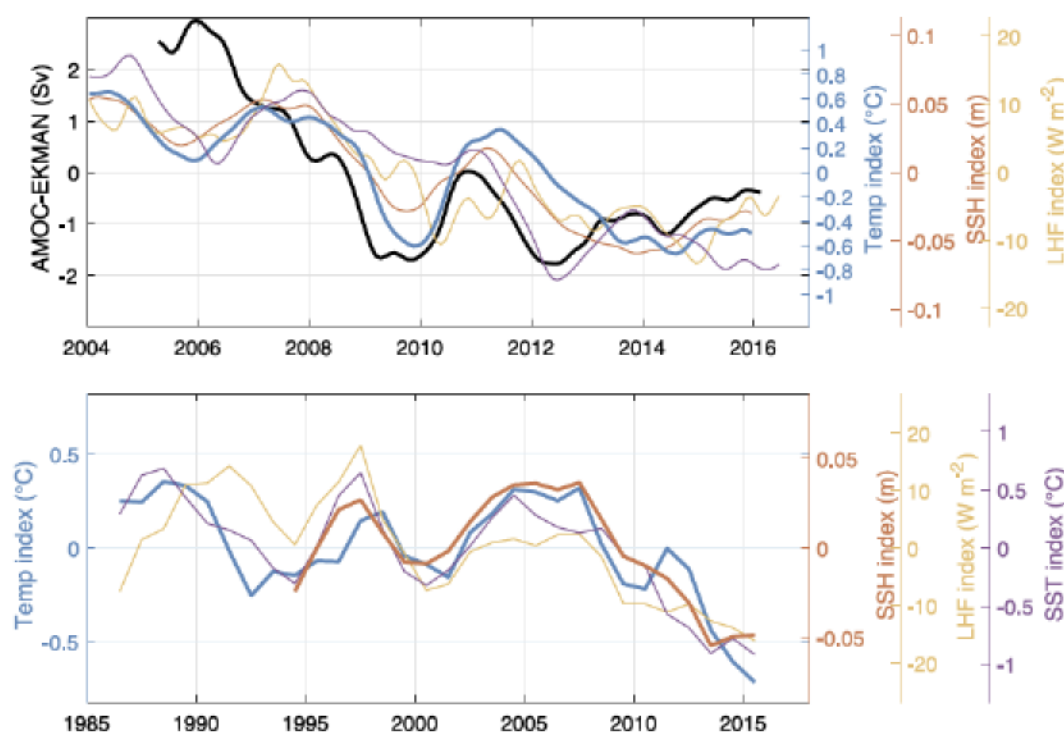
Figure 3. Indices of subsurface temperature, sea surface height (SSH), latent heat flux (LHF), and sea surface temperature (SST). SST (purple) is plotted using the same scale as subsurface temperature (blue) in the upper panel. The upper panel shows 24 month filtered values of de-seasonalized anomalies along with the non-Ekman part of the AMOC. In the lower panel, we show three-year running means of the indices going back to 1985 (1993 for the SSH index).
