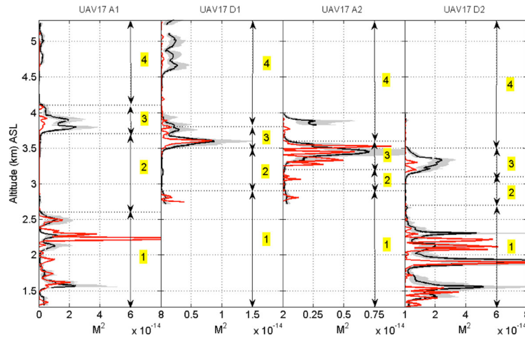
Fig. 8 Comparisons between M^2_{UAV} (red) and M^2_{rad} (black) profiles in linear scales for A1, D1, A2, and D2 flight phases of UAV17. The labels (1) to (4) refer to the region emphasized in Fig. 5b. Horizontal scales have been adapted to the dynamics of the values
