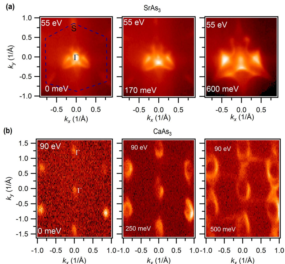
Figure 2. Fermi surface and constant energy contours of \text{RAS}_3 (a) Fermi surface and constant energy contour plots of \text{SrAs}_3 , measured at the ALS beamline 10.0.1 using a photon energy of 55 eV. (b) Measured Fermi surface and constant energy contour plots of \text{CaAs}_3 . Each of the distorted hexagons represents a separate Brillouin zone where the b-axis is larger than the a-axis. The measurements were performed at the HRPES end-station of the SLS beamline at a temperature of about 18 K using an incident photon energy of 90 eV. The binding energies are marked in the plots.
