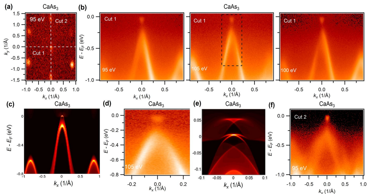
Figure 4. Dispersion maps along the high symmetry directions in \text{CaAs}_3 . (a) Fermi surface map at a photon energy of 95 eV. White dashed line guides the energy-momentum dispersion measurement directions. (b) Photon energy dependent dispersion maps along the cut 1 direction shown in Fig. 4(a). (c) Calculated dispersion map without the inclusion of SOC around the Y point of BZ. At the (010) surface, Y and \Gamma are projected at the same point. (d) Zoomed in plot of black dashed box shown in 105 eV dispersion map. (e) Calculated zoomed-in plot near the Fermi level. (f) Measured dispersion map along the cut 2 direction at a photon energy of 95 eV.
