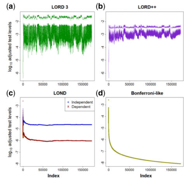
Fig. 1. Adjusted significance thresholds on the log10 scale. Applied to genotype effect data from the IMPC dataset, at a FDR level of 5%. (a) LORD 3, (b) LORD++, (c) LOND and (d) Bonferroni-like
