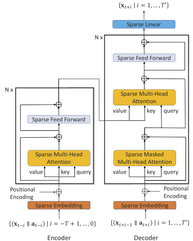
Figure 3. Architecture of Forecaster ( a \parallel b represents concatenating vector a with vector b ).
