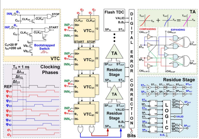
Figure 10.8.2: Circuit realization of the 4-element SSP (center); including the voltage-to-time converter (VTC, top left); time-amplifier (TA, top right); clocking phases (bottom left); and residue stage (bottom right).
