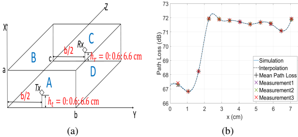
Fig. 2. Exploration of LoS propagation in an empty metal cavity at 300 GHz for 2-D case: (a) Measurements setup, (b) Comparison of theoretical and measured path loss with respect to transceiver's height.
