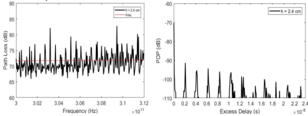
Figure 2. (left) Path loss vs frequency and (right) measured PDP for a cavity with the dimension of 30.5 cm × 10 cm × 10 cm.
