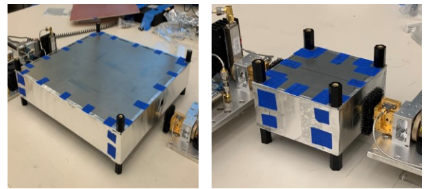
Figure 1. Rectangular metallic cavities used in measurements (left) larger cavity of dimension 30.5 \times 30.5 \times 5cm (right) small cavity 11 \times 11 \times 5cm.
