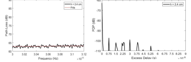
Figure 4. (left) Path loss vs. frequency and (right) measured PDP for a smaller size box.
