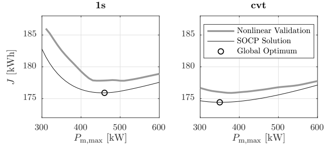
Fig. 6. Solution of Problem 1 for different values of P_{m,\max} (SOC Solution) and validation through simulation in the nonlinear model (Nonlinear Validation) for the long-haul driving cycle. For both the single-gear (1s) and the CVT the nonlinear model simulation results in slightly higher values. Yet, the trends are in line with each other.
