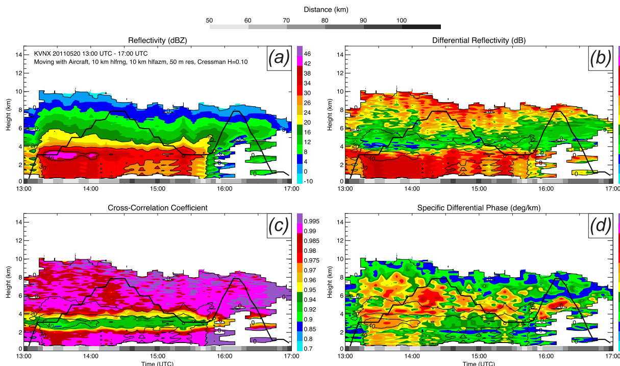
FIG. 9. Moving CVP using measurements from the KVNx radar from 1300 to 1700 UTC 20 May 2011. The CVP sector moved with the location of the research aircraft flying during the MC3E campaign. (a) Z , (b) Z_{DR} , (c) \rho_{hv} , and (d) K_{DP} . The bold black line overlaid in each panel represents the altitude of the aircraft with time, and thin black lines represent reflectivity at 0, 20, 30, and 40 dBZ. Vertical data spacing in the CVP is 50 m, and the sector size is 20 km in range and 20^\circ in azimuth. Distance from the radar for each scan is denoted just above the x axis on each panel.
