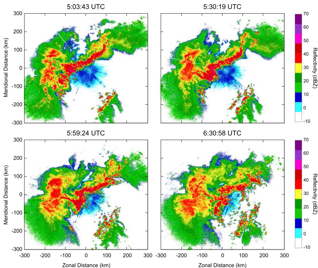
FIG. 2. PPI images of radar reflectivity (dBZ) collected at the 0.5^\circ elevation angle by the KFSD radar from 0500 to 0630 UTC. Images were selected at approximately half-hour intervals, with specific times of data collection listed above each panel.
