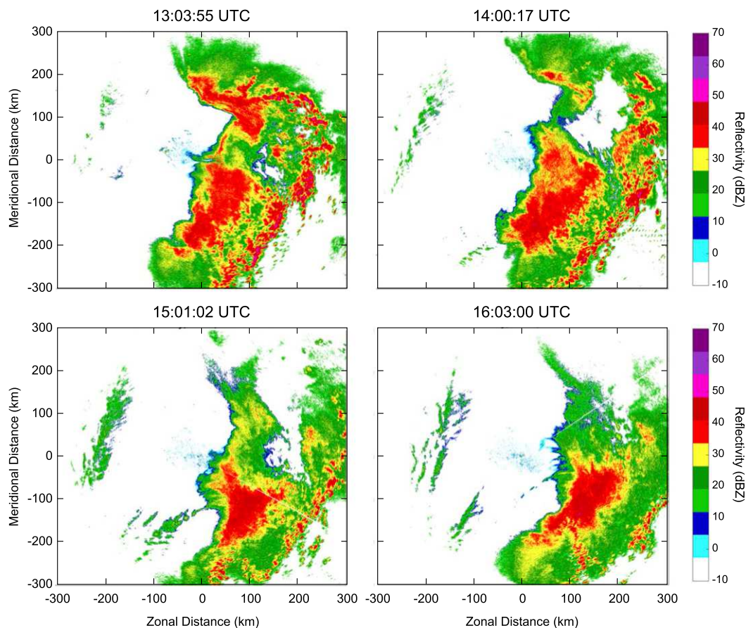
FIG. 1. PPI images of radar reflectivity (dBZ) collected at the 0.5^\circ elevation angle by the KVN radar from 1300 to 1600 UTC. Images were selected at approximately 1-h intervals, with specific times of data collection listed above each panel.
