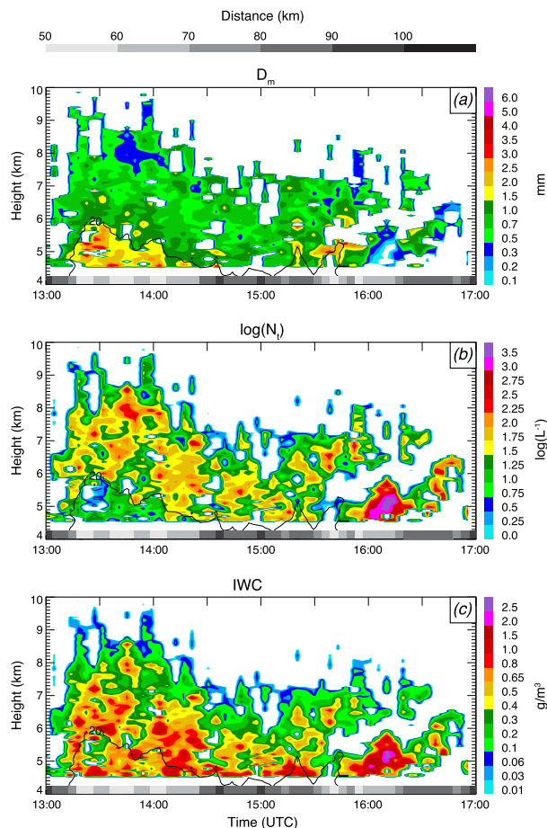
FIG. 12. Ice microphysical retrievals performed on the 20 May 2011 moving CVP. Plots show (a) D_m (mm), (b) \log(N_t) [ \log(L^{-1}) ], and (c) IWC ( g m^{-3} ). Retrieval data shown herein are limited to altitudes above 4.5 km. Thin black lines represent reflectivity at 20 dBZ. Distance from the radar for each scan is denoted just above the x axis in each panel.
