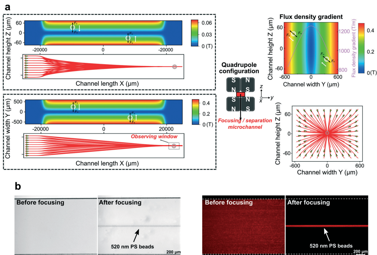
Fig. 2 System optimizations of the FerroChip for continuous-flow nanoparticle focusing. a Optimization of high magnetic flux densities and high magnetic flux density gradients in the FerroChip for nanoparticle focusing. Using four permanent magnets (38.1 mm by 6.35 mm by 6.35 mm, N52 neodymium magnet) in a quadrupole configuration shown here, a magnetic flux density of up to 0.5 T in the x - y plane ( z = 0 ), and a magnetic flux density gradient of 1272\ \text{T m}^{-1} in the y - z plane ( x = 0 ) were obtained. Under the magnetic field of the quadrupole magnets, simulation of submicron particle trajectories for 520 nm polystyrene beads in ferrofluids in x - y plane (left), x - z plane (middle), and y - z plane (right), were conducted to study the effectiveness of FerroChip in focusing 520 nm diamagnetic beads. A sample inlet flow rate of 3\ \mu\text{L min}^{-1} and a ferrofluid concentration of 0.3% (v/v) were used in the simulation. Results show that 520 nm beads could be focused in all three dimensions in the prototype device. Triangles in the trajectory plots indicate the starting points of particles. b (Left panel) Experimental bright-field images show that 520 nm diamagnetic polystyrene beads inside a microchannel can be focused into a narrow stream in the presence of the ferrofluid and quadrupole magnets, using optimized parameters from a . (Right panel) Experimental fluorescence images confirm the focusing effects on 520 nm polystyrene. A sample inlet flow rate of 3\ \mu\text{L min}^{-1} and a ferrofluid concentration of 0.3% (v/v) were used in b . Scale bar: 200 \mu\text{m} .
