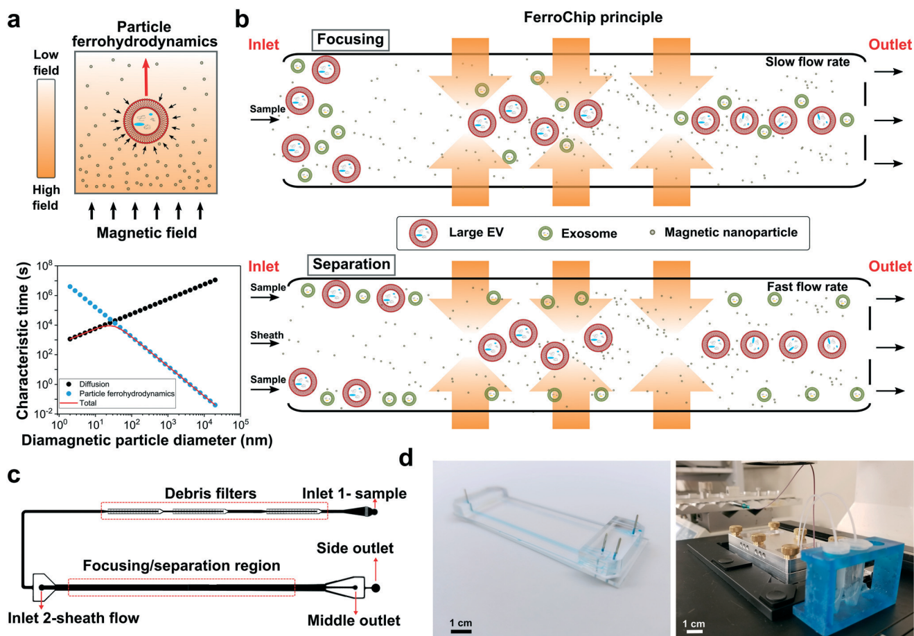
Fig. 1 Overview of the label-free ferrohydrodynamic nanoparticle separation principle and the FerroChip device design. a (top panel) Schematic of an extracellular vesicle (EV, 30–1000 nm in diameter) experiencing both diffusion and “particle ferrohydrodynamics” in a colloidally-stable magnetic nanoparticle (~10 nm particle diameter) suspension ( i.e. , ferrofluids). The magnetization of the unlabeled EV M_{EV} is near zero and much less than its surrounding ferrofluids M_{ferrofluid} . The ferrohydrodynamic force on the EV is generated from magnetic nanoparticle-induced pressure imbalance on the vesicle’s surface, which is proportional to the EV’s volume. The color bar indicates the relative amplitude of the magnetic field strength. Red arrows show the direction of vesicle movement, small black arrows on the EV’s surface show the direction of magnetic nanoparticle-induced surface pressure. (bottom panel) The relationship between characteristic migration time of a diamagnetic nanoparticle in ferrofluids and the diameter of the nanoparticle. The migration of nanoparticles is affected by both diffusion and “particle ferrohydrodynamics”, and determined by the faster process out of the two. For nanoparticles with a diameter of less than ~30 nm, the diffusive process dominates the migration; for nanoparticles with a diameter of larger than ~30 nm, the ferrohydrodynamic process dominates the migration. b Work principle of a label-free continuous-flow EV focusing/separation device, termed as FerroChip. In the focusing mode of device operation, samples of EVs were premixed with a dilute ferrofluid and entered a straight microchannel at a relatively slow flow rate and with a uniform distribution across the channel width. A symmetric magnetic field with its minimum in the middle of the microchannel was used to direct EVs towards the center of the microchannel, effectively focusing them into a narrow stream. In the separation mode, EVs entered the channel predominately through the regions close to the channel wall due to a sheath flow, with a relatively fast flow rate. The same magnetic field was used to direct unlabeled EVs from the sidewall region towards the channel center for continuous collection. EVs of various sizes migrated towards the center of the microchannel, with varying speeds that depended on their sizes. Large EVs migrated to the channel center at a faster speed than smaller exosomes. Yellow arrows with gradients indicate the distribution of magnetic fields in the microchannel. c Top-view schematic drawing of the FerroChip’s microchannel. Initial samples of nanoparticles and/or EVs were injected into the channel from inlet 1. The samples, after first going through a debris filter that removed large debris, entered a straight channel (labeled as focusing/separation region) which focused or separated nanoparticles and/or EVs based on their sizes. Processed samples were collected from middle and side outlets for characterizations. When the FerroChip operates in focusing mode, inlet 2 (sheath flow) is not used. When the FerroChip operates in separation mode, inlet 2 provides a ferrofluid sheath flow so that nanoparticles and/or EVs entered from the top and bottom walls of the channel. The width, height and length of the microchannel are 1200 \mu\text{m} , 150 \mu\text{m} and 53 mm, respectively. d A photo of a microchannel (left, blue ink indicating the channel geometry) and assembled FerroChip with four permanent magnets in quadrupole configuration inside a holder (right). The microfluidic device and permanent magnets were placed within an aluminum manifold during its operation. Scale bars: 1 cm.
