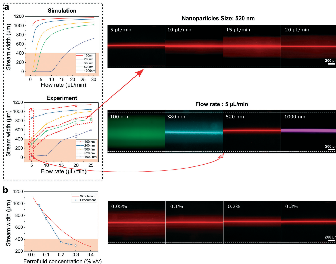
Fig. 3 Optimizations of nanoparticle focusing in the FerroChip, with parameters including particle diameter, flow rate, and ferrofluid concentration. a Optimizations of nanoparticles focusing with parameters including nanoparticle diameters and flow rates through both simulations and experiments. Simulation results agreed with experimental results reasonably well. Both confirmed that the ferrohydrodynamic focusing effect on nanoparticles depended on the diameters of particles in ferrofluids. As the particle size increased, the focusing effect became more pronounced. Additionally, as the flow rates in the microchannel increased, the focusing effect decreased. Particle stream width of the y-axis label indicates the width of the focused particle stream. Orange color shaded area indicates the width of the collection outlet in the FerroChip. A panel of fluorescent images captured during the focusing of 100 nm, 380 nm, 520 nm, and 1000 nm polystyrene beads at a flow rate of 5 \mu\text{L min}^{-1} illustrates that focusing effect depended on particle sizes. b Optimizations of nanoparticles focusing with the parameter of ferrofluid concentration through both simulations and experiments. Simulation results agreed with experimental results reasonably well. Both confirm that the ferrohydrodynamic focusing effect on submicron beads depended on the ferrofluid concentration. As the ferrofluid concentration increased, the focusing effect became more pronounced. A panel of fluorescent images captured during the focusing of 520 nm polystyrene beads at 0.05%, 0.1%, 0.2% and 0.3% (v/v) ferrofluid concentration illustrates that focusing effect depended on ferrofluid concentrations. Flow rate was 5 \mu\text{L min}^{-1} . Scale bar is 200 \mu\text{m} in all images.
