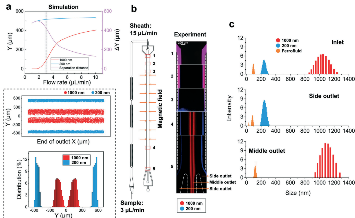
Fig. 4 Optimizations of the FerroChip for the separation of exosome-like nanoparticles (30–150 nm in diameter) from large extracellular vesicles (200–1000 nm in diameter). a Simulation results of the separation of 200 nm and 1000 nm polystyrene beads, at different flow rates (1–10 \mu\text{L min}^{-1} ) in a 0.3% (v/v) ferrofluid. We considered 1–3 \mu\text{L min}^{-1} to be optimal flow rates because they correspond to more than 400 \mu\text{m} separation distance in simulation. A 3 \mu\text{L min}^{-1} optimal flow rate was chosen to separate 200 nm and 1000 nm polystyrene beads from each other. The ratio of particle flow and sheath flow was 1:5 (sample – 3 \mu\text{L min}^{-1} ; sheath – 15 \mu\text{L min}^{-1} ). Other simulation parameters included a ferrofluid concentration of 0.3%, and the same quadrupole magnet configuration in previous figures. Using these parameters, we simulated the distribution of 200 nm and 1000 nm beads at the outlets of the FerroChip. Particle trajectories from the simulation results predicted that the two differently sized particles could be completely separated. b Experimental images of the separation of a mixture of 200 nm (blue) and 1000 nm (red) polystyrene particles in the FerroChip. Fluorescent images taken at different locations along the microchannel showed that 200 nm particles (blue) were completely separated from 1000 nm particles (red). Both particles were collected for subsequent size characterization. Broad blue fluorescent signals across the channel at the location #3 were from the shade of the permanent magnets, not fluorescent particles. c Particle size distributions measured by dynamic light scattering (DLS) indicate a well-separated 1000 nm and 200 nm particles after FerroChip processing.
