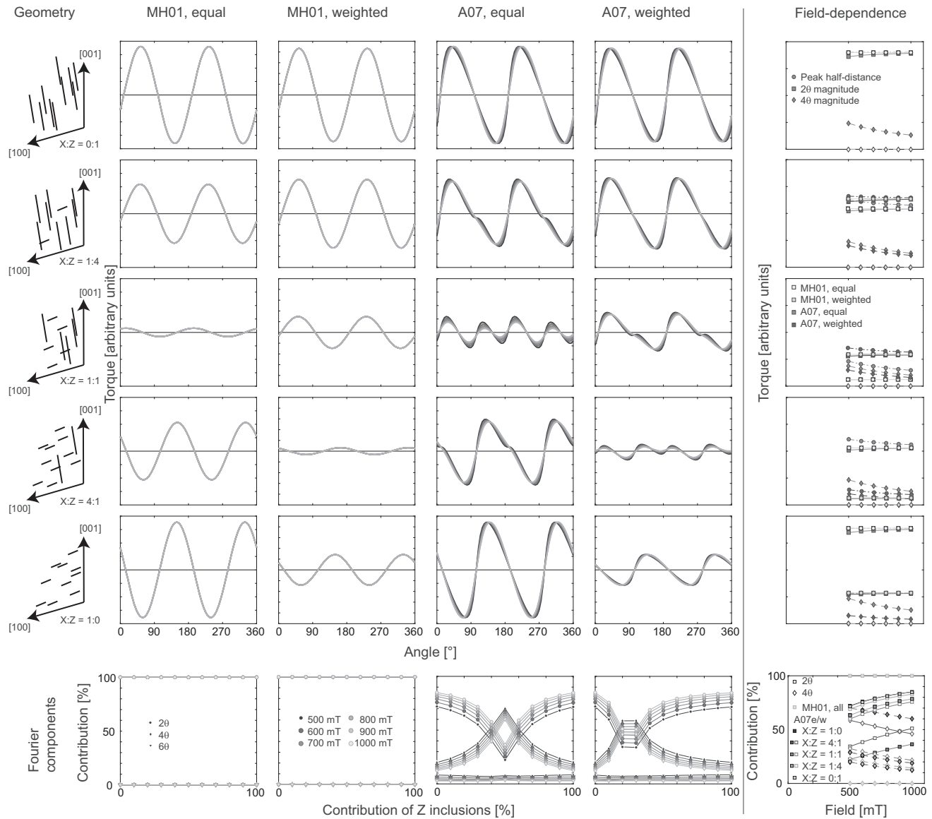
Figure 10. Expected torque curves, Fourier components, and field dependence for a single clinopyroxene crystal with various proportions of X and Z inclusions. All results shown for the [100]–[001] plane.
