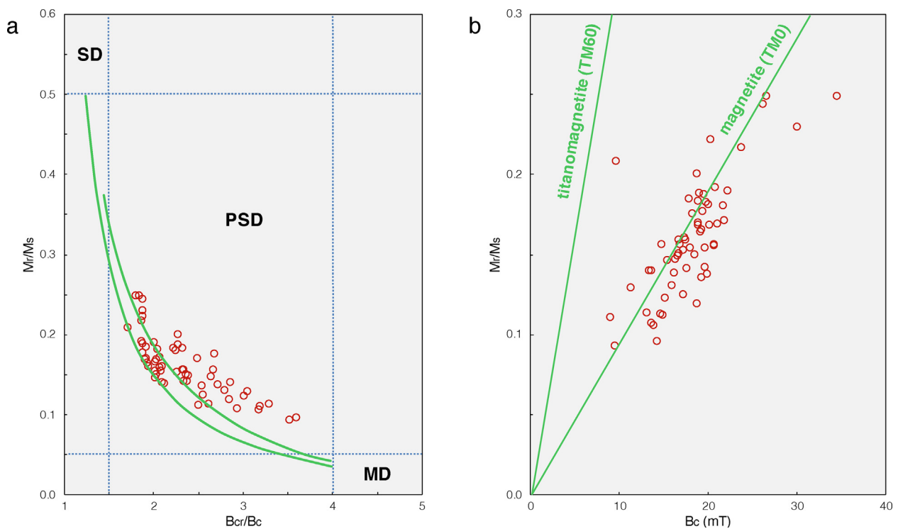
Fig. 8. (a) Day plot ( B_{cr}/B_c vs. M_r/M_s ) of the NG1 obsidian artifacts with magnetic domain boundaries (dotted blue lines) and magnetite mixing curves (solid green lines) from Dunlop (2002). All artifacts fall in the pseudo-single domain (PSD) region of the plot, not the single domain (SD) or multi-domain (MD) regions. Magnetite grains exhibit PSD behavior in the 0.1 to 20 \mu\text{m} size range. (b) NG1 artifact data ( B_c vs. M_r/M_s ) with the compositional lines for magnetite (TM0) and titanomagnetite (TM60) based on calculations by Wang and Van der Voo (2004).
