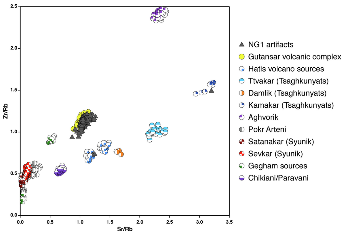
Fig. 9. A scatterplot of \text{Sr}/\text{Rb} vs. \text{Zr}/\text{Rb} (i.e., \text{Sr} vs. \text{Zr} normalized to \text{Rb} ) for the geological obsidian specimens and the NG1 small debris in this study. This scatterplot is directly comparable to Fig. 7a in Frahm et al. (2016:84).
