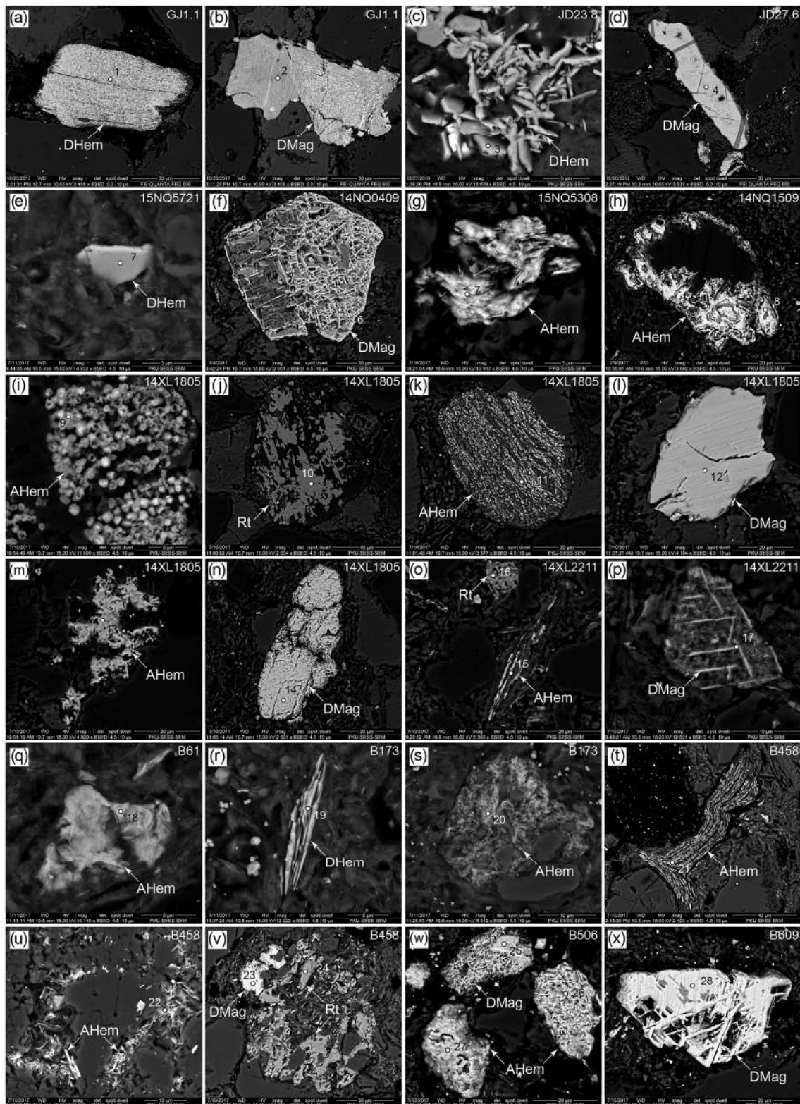
Figure 10. SEM backscattered electron images of samples from the Gongjue, Nangqian, Shanglaxiu, and Jinggu basins. DHem = detrital hematite; AHem = authigenic hematite; DMag = detrital magnetite; Rt = rutile. (a–d) From samples retaining a DRM from the Gongjue Basin; (e) from a Type C sample retaining a DRM from the Nangqian Basin; (f–h) from remagnetized Types A and B samples from the Nangqian Basin; (i–p) from remagnetized samples from the Shanglaxiu Basin; and (q–x) from remagnetized samples from the Jinggu Basin. Dots represent spots for EDS analysis with the results presented in Figure S1.
