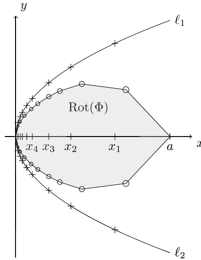
FIGURE 1. The rotation set defined in Example 7.1. The rotation set is an infinite polygon and the origin is an exposed point.
