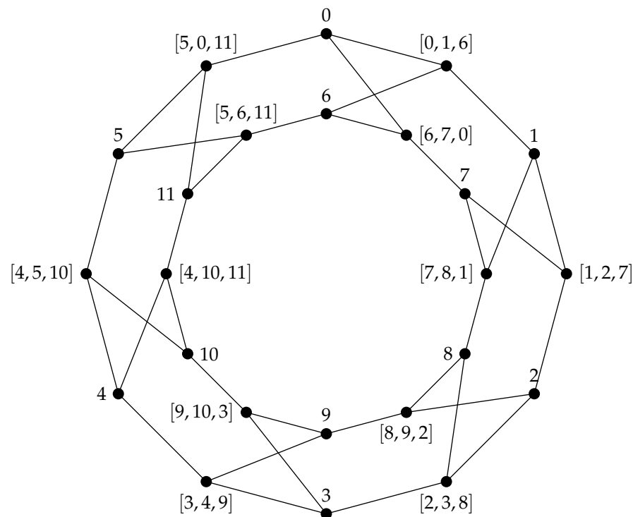
Figure 2. A half-step graph G_{24}[0, 1, 6] .
