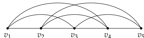
Figure 1. The graph P_5^3 .
