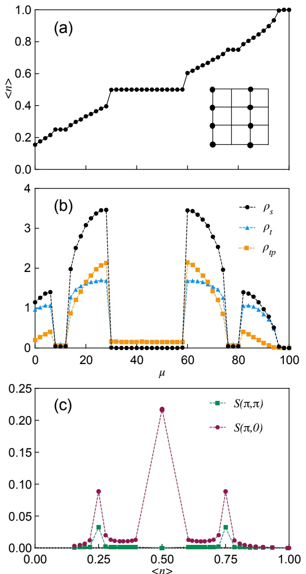
FIG. 5. (a) Plot of boson density \langle n \rangle , (b) plot of total stiffness \rho_s , single stiffness \rho_t and pair stiffness \rho_{tp} , (c) plot of S(\pi, \pi) and S(\pi, 0) . Parameters for this simulation are t_p = 4 , V = 6 , V_d = 10 for a L = 12 system.
