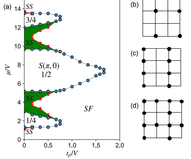
FIG. 4. (a) Ground-state phase diagram of Eq. (1) with t/V = 1/6 and V_d/V = 5/3 . Three distinct Mott insulating lobes are present with their densities indicated, as well as supersolid and superfluid phases. Illustrations of the ground state configuration of the (b) \frac{1}{4} , (c) \frac{1}{2} and (d) \frac{3}{4} solids on a L = 4 lattice.
