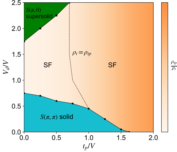
FIG. 3. Ground-state phase diagram of Eq. (1) at t/V = 1/4, \mu/V = 5 . Lines are guide to the eyes. The dotted line indicates the boundary where \rho_t = \rho_{tp} . The orange intensity represents the magnitude of the ratio \rho_{tp}/\rho_t , which increases with t_p . A S(\pi, 0) solid is stabilized at larger \mu/V and is not shown in this phase diagram.
