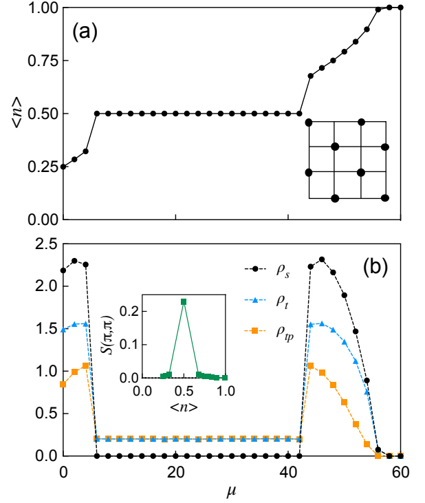
FIG. 7. The boson density (a) and the various stiffness constants (b) as functions of \mu . The inset of (a) illustrates the geometry of bosons at the \langle n \rangle = \frac{1}{2} checkerboard plateau. The inset of (b) plots S(\pi, \pi) as a function of boson density. Parameters for this simulation are t_p = 4, V = 6, V_d = 0 for an L = 8 system.
