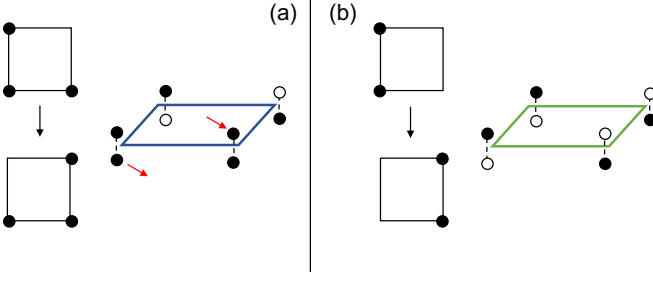
FIG. 2. An illustration of the creation of a pair hopping operator through a loop update. The operator string propagation level propagates downwards in this figure. (a) The left shows a single hop operator in real space as the lattice is propagated in imaginary time. The right shows the 3D representation of a 8-legged vertex, with a single hop operator represented by a blue rectangle. Filled circles represent a boson and empty circles represent empty sites. The red arrows indicate the introduction of a defect into and out of the vertex as part of the loop update. Propagation of defects cause a boson occupancy inversion. (b) The left shows the resulting pair hop operator acting in real space. The right shows the pair hop operator as a result of the loop update, represented by a green rectangle. Note that to obtain the pair hop operator, we simply flip the boson occupancy of the two sites indicated by red arrows in (a), which was initially a single-hop operator. This occupancy flip resulted in the conversion from a single-hop operator to a pair-hop operator.
