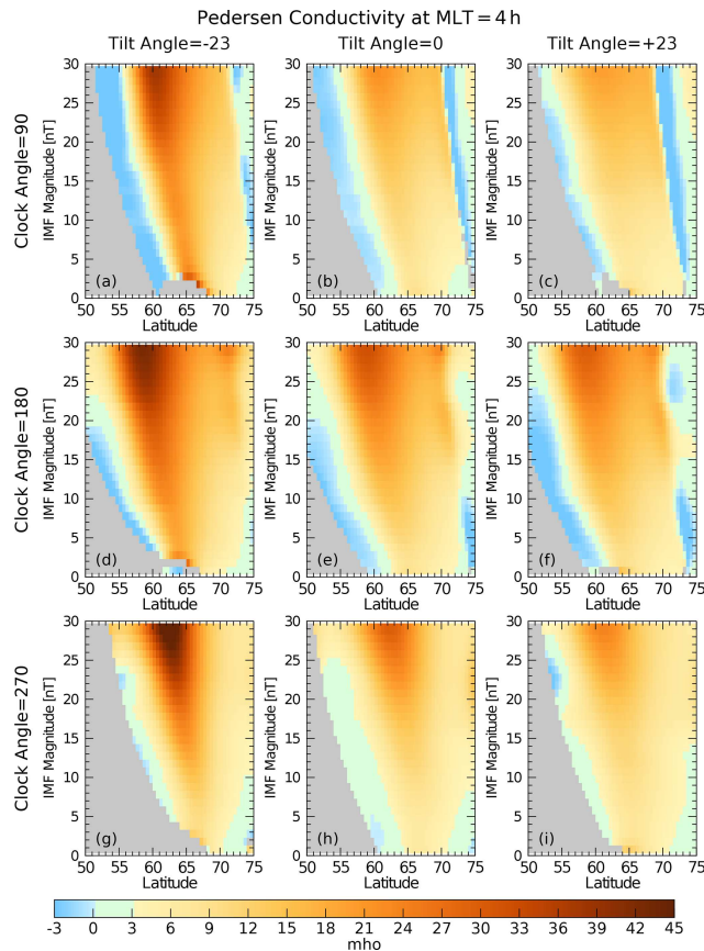
Figure 6. Pedersen conductivity as a function of latitude from 50 to 75° at 4:00 MLT. Values were calculated for IMF magnitudes of 1 to 29 nT, at 1 nT intervals, indicated on the ordinate. Multiple graphs are shown for dipole tilt angles of -23^\circ (a, d, g), 0^\circ (b, e, h), and +23^\circ (c, f, i) and IMF clock angles of 90^\circ (a, b, c), 180^\circ (d, e, f), and 270^\circ (g, h, i). Conductivity values are colored according to the scale at the bottom. Gray and blue areas indicate invalid results, as noted in the text.
