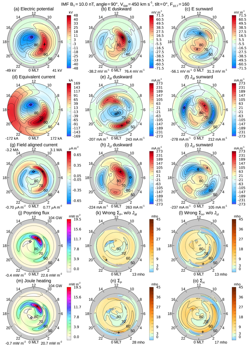
Figure 4. Conductivity input data and results for the same conditions as in Fig. 1, except that IMF clock angle is changed 90^\circ . The IMF B_T magnitude is 10 nT, the solar wind velocity is 450 km s ^{-1} , the F_{10.7} index is 160 sfu, and the dipole tilt angle is 0^\circ .
