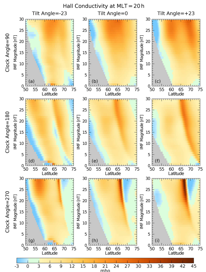
Figure 9. Hall conductivity as a function of latitude from 50 to 75° at 20:00 MLT. The format of the graph is the same as in Figs. 6 to 8.
