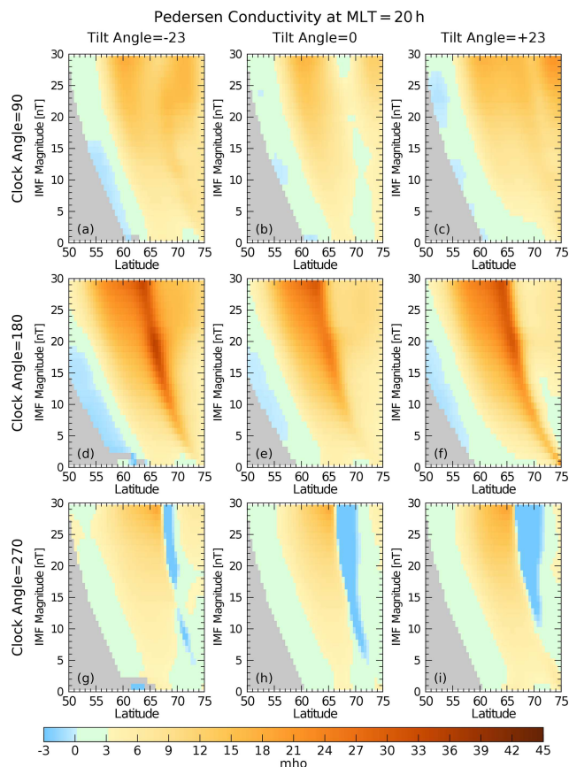
Figure 8. Pedersen conductivity as a function of latitude from 50 to 75° at 20:00 MLT. The format of the graph is the same as in Fig. 6, with only a change in the MLT.
