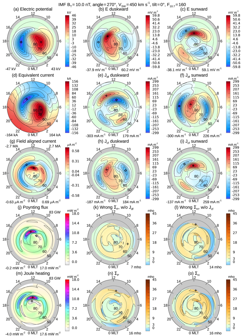
Figure 5. Conductivity input data and results for the same conditions as in Fig. 1, except that IMF clock angle is changed 270^\circ . The IMF B_T magnitude is 10 nT, the solar wind velocity is 450 km s ^{-1} , the F_{10.7} index is 160 sfu, and the dipole tilt angle is 0^\circ .
