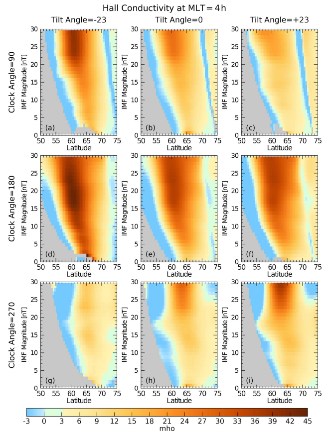
Figure 7. Hall conductivity as a function of latitude from 50 to 75° at 4:00 MLT. The format of the graph is the same as in Fig. 6.
