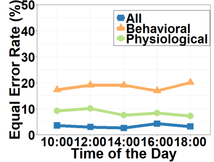
Fig. 15: The EERs are stable in the one-day short-term period.
