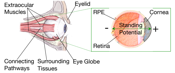
Fig. 1: HVS structure (left) and standing potential (right).
