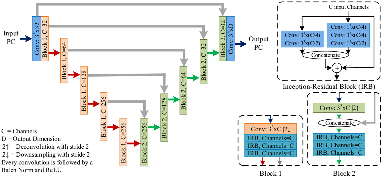
Fig. 4: Network Architecture.
