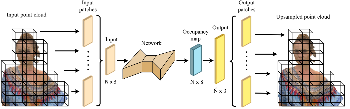
Fig. 2: System Model.
