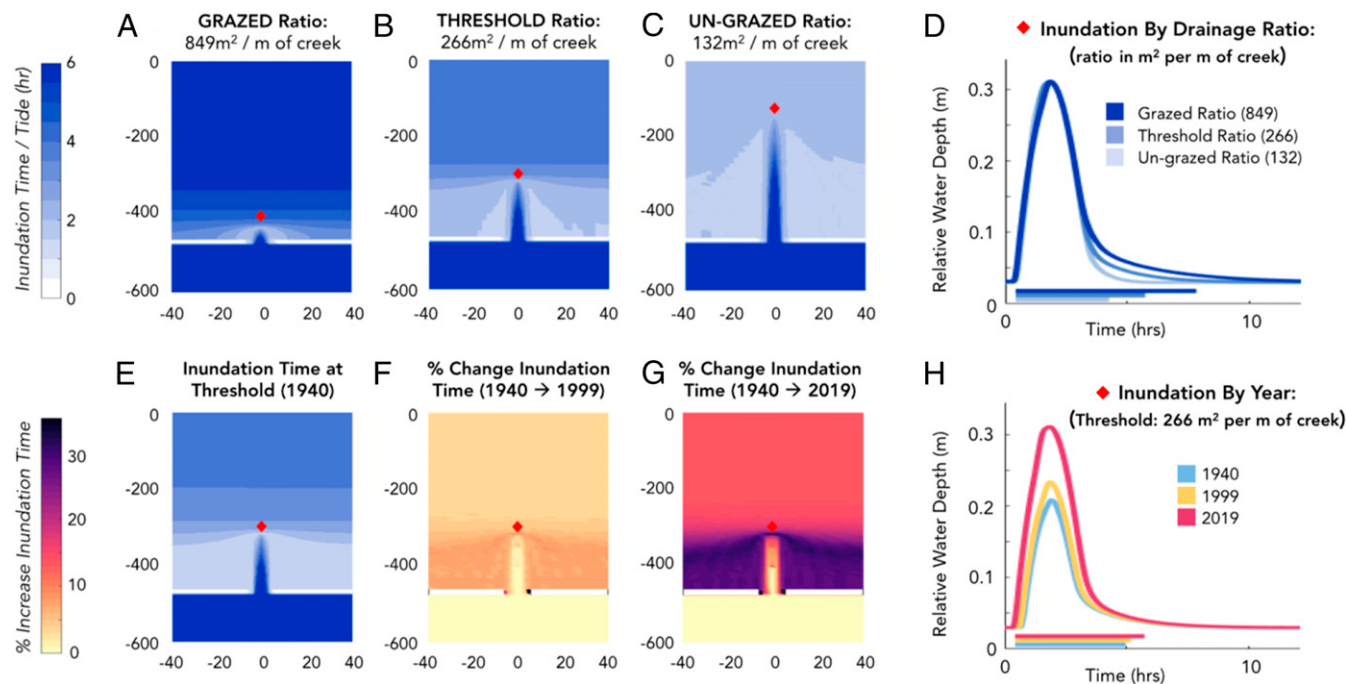
Fig. 3. ROMS simulations. (A–C) ROMS simulations were conducted by using three idealized model bathymetries that differed only in the length of the tidal creek, such that their drainage ratios were those of grazed (A; 849 m 2 per m of tidal creek), threshold (B; 266 m 2 per m of tidal creek), and ungrazed conditions (C; 132 m 2 per m of tidal creek). Submergence, or inundation time, is presented on a scale of blue color, with darker hues representing longer periods of submergence. In all panels, a location standardized for elevation (+0.70 m ASL) and proximity to tidal creekhead (20 m) is shown as a red diamond. (D) Inundation time at this reference point is presented for the three bathymetries. (E) Adjusting the elevation of the threshold simulation for relative rates of sea-level rise, inundation time is presented for the threshold drainage ratio in 1940. (F and G) Percent increases in inundation time between 1940 and both 1999 (F) and 2019 (G) are depicted on a color scale of yellow (low) to red (intermediate) to purple (high). (H) Changes in inundation time at the reference point are shown between 1940, 1999, and 2019.
