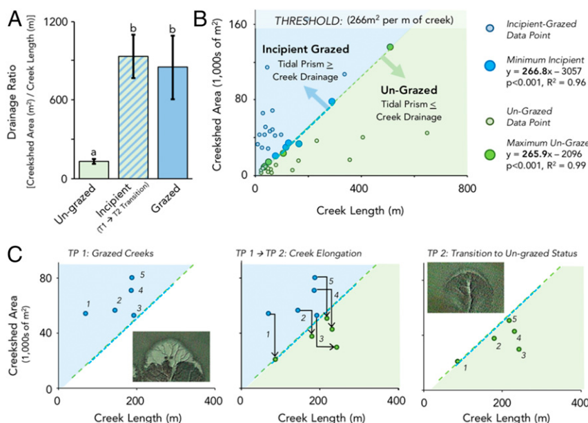
Fig. 2. Geospatial drivers of Sesarma -grazed creekhead distribution. (A) Drainage ratios of grazed and incipient-grazed creeks were six times higher than those of ungrazed creeks. (B) Marginal incipient-grazed creeks (five minimum drainage ratios) and ungrazed creeks (five maximum drainage ratios) were assessed by using linear regression analyses. Results identified a threshold drainage ratio of 266 m 2 per m tidal creek (dashed blue and green regression lines). Above this line, we suggest that the volume of water that requires drainage per tidal cycle (i.e., tidal prism) is greater than the creek-drainage capacity, and, as a result, grazing is likely to initiate. Below this line, the creek’s hydraulic capacity is sufficient to drain the adjacent marsh platform, and the creek remains ungrazed. (C) Five creeks with a history of grazing at TP1 that transitioned to an ungrazed status at TP2 show that this transition away from grazing coincides with the creek transitioning from above to below the identified threshold drainage ratio.
