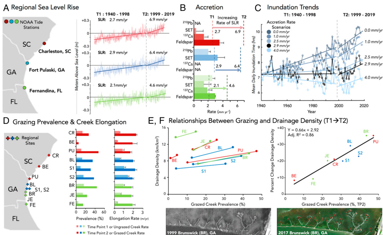
Fig. 1. Sea-level rise, submergence, and Sesarma -grazing trends. (A) Relative sea-level rise recorded at the Charleston, SC (northern; red); Fort Pulaski, GA (central; blue); and Fernandina Beach, FL (southern; green) NOAA tide stations from 1940 to 2019. Trend lines and black text denote the average annual rate of sea-level rise (SLR) during the 1940 to 1998 (T1) and 1999 to 2019 (T2) time periods. (B) Rates of salt-marsh-platform vertical accretion measured via ^{210}\text{Pb} , SET, ^{137}\text{Cs} , and Feldspar marker horizon methods are shown as mean \pm SE for each method for salt marshes located in each subregion. Dashed lines refer to the relative rate of sea-level rise in each subregion at T1 and T2. (C) First-order approximations of the duration of tidal submergence, or inundation time (hours per day), experienced by salt-marsh creekheads under each of five marsh vertical accretion-rate scenarios. The dashed gray line denotes the boundary of T1 and T2. (D) Aerial-image analysis of 1-km 2 areas at each of nine sites (site name abbreviations are reported inset and across panels) revealed that grazed creek prevalence increased at all sites between TP1 (light shading) and TP2 (dark shading) and that the elongation rate between the two time points is faster for grazed creeks than ungrazed creeks in all locations. (E) At all sites, marsh-drainage density increased with the rise in grazed creek prevalence observed between TP1 and TP2. (F) Across all sites, grazed creek prevalence at TP2 strongly predicted the percent change in drainage density between the two time points. Model results are presented (inset) and aerial images depicting changes in creek length between TP1 and TP2 are shown (E and F, Lower).
