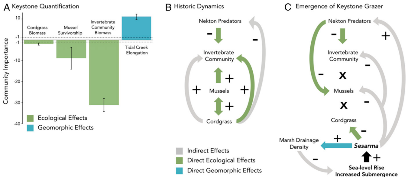
Fig. 6. Sesarma 's community importance and effects on salt-marsh interaction networks. (A) Sesarma 's community importance in controlling cordgrass biomass, mussel survivorship, macrobenthic invertebrate community biomass, and creek elongation, averaged across border and platform zones at the three Sapelo Island sites. All data are shown as mean \pm SE of a minimum of 24 replicate measurements per grazed and ungrazed creekshed assessed for each factor. Positive community importance reflects an increase in the metric, while negative values reflect a decrease in the metric when Sesarma are present in higher density (grazed creeks) as compared to lower densities (ungrazed creeks). Species with community importance values far greater than \pm 1 (denoted by dashed lines) are considered "keystone" species. (B and C) Conceptual diagram summarizing the likely differences in species interaction networks in southeastern US Atlantic salt marshes in this "historic" period of 1940 to 1999 (B) vs. the contemporary period of 1999 to 2019 when Sesarma -grazed creeks have become prevalent features (C) due to Sesarma 's direct and indirect effects (colored and gray arrows, respectively) on other community members.
