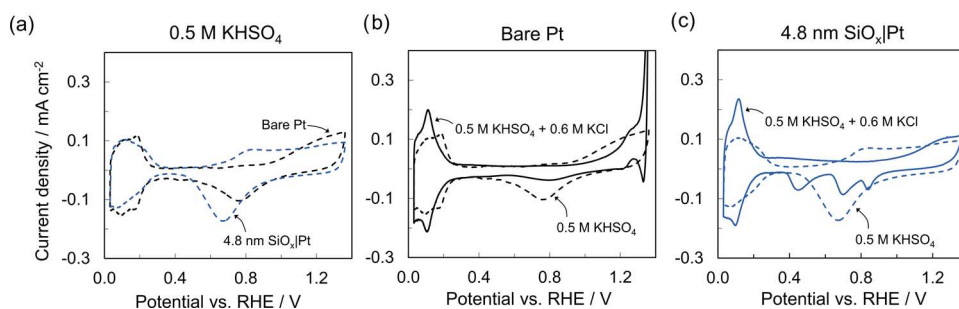
Figure 2. CV measurements for (a) bare Pt (black curves) and 4.8 nm SiO x |Pt (blue curves) in 0.5 M KHSO 4 . CV measurements for (b) bare Pt and (c) 4.8 nm SiO x |Pt in 0.5 M KHSO 4 (dashed curves) and 0.5 M KHSO 4 + 0.6 M KCl (solid curves). All measurements were performed at 100 mV s -1 in deaerated electrolyte at pH 0.8 and 25 °C.
