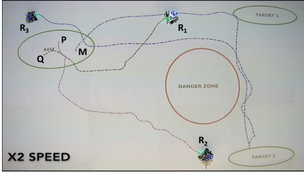
Figure 3: A still shot of the trajectories for the robots R_1 , R_2 , and R_3 for the specification \phi as in (39). Observe that R_1 moves temporarily away from target 1 temporarily in order to satisfy the connectivity constraint, but Theorem 1 results in feasible solutions at those points. From the figure, we observe that the robots maintain connectivity and avoid the danger zone at all times.
