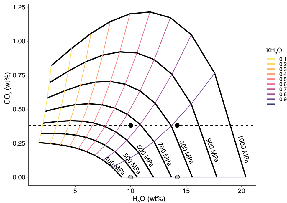
Fig. 11 \text{H}_2\text{O} and \text{CO}_2 solubility using the model of Papale et al. (2006) using the composition of enclave 17-06A and a temperature of 1100 °C at a variety of pressures (400–1000 MPa) and fluid compositions ( X_{\text{H}_2\text{O}} ). Dashed line is at 3800 ppm \text{CO}_2 , the estimated \text{CO}_2 content of Klyuchevskoy from melt inclusions (Mironov et al. 2015). Grey dots represent the range of estimated water content from P_{\text{H}_2\text{O}} and black dots represent minimum pressure estimates of amphibole
