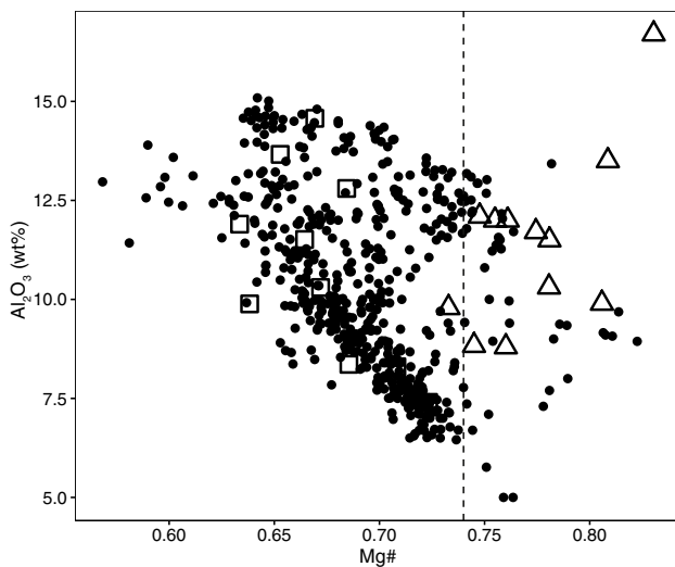
Fig. 6 Amphibole phenocryst variation diagram in \text{Al}_2\text{O}_3 . Open triangles represent analyses of inclusions of amphibole in olivine and open squares represent analyses of inclusions of amphibole in plagioclase. Dashed line is placed at \text{Mg}\# = 74 ; analyses to the right of the line were those used in amphibole barometry
