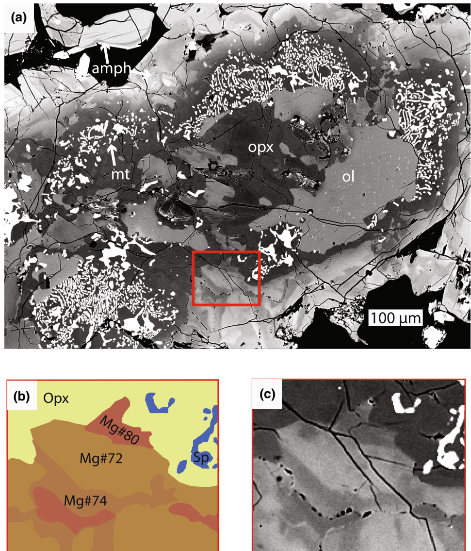
Fig. 5 a BSE image of heavily reacted symplectite grain. b Line diagram of outer amphibole reaction rim (brown/orange) and inner orthopyroxene reaction rim from area outlined in red in a . c BSE image of the area depicted in b
