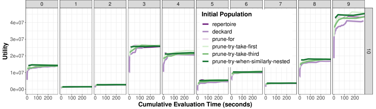
Fig. 5: Utility versus planning time for the four beneficial syntactic transforms. Some transforms obtained results as quick as Deckard but with better utility. try-take-first is the overall best after around 2 minutes of planning.
