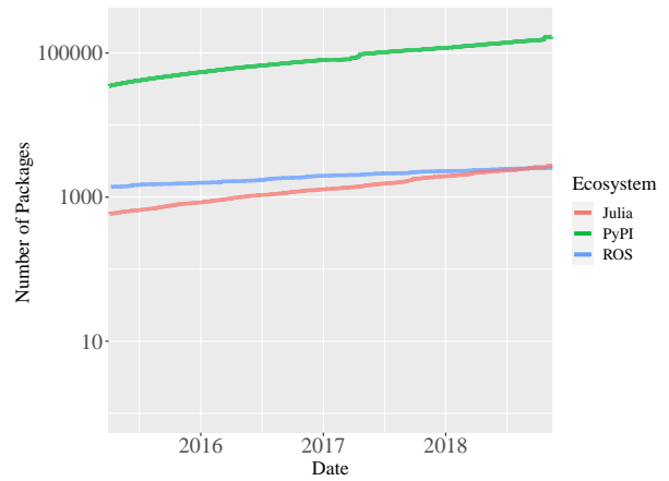
Fig. 3. Growth of the ROS (Kinetic), PyPI, and Julia ecosystems, in terms of number of packages, plotted on a log scale. For each of these curves, the most explanatory regression was linear, as opposed to exponential.
