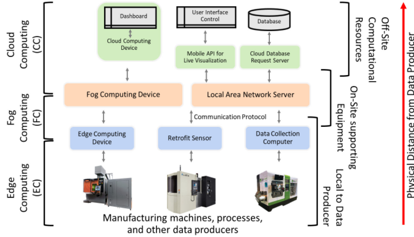
Figure 1: Diagram of connections and physical locations of Edge Computing (EC), Fog Computing (FC), and Cloud Computing (CC) devices with relation to data producers. EC, FC, and CC devices are distinguished based on physical proximity to the data source.
