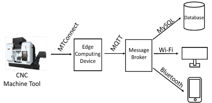
Figure 2: Example data transmission framework with mixed communication protocols. MTConnect provides initial data acquisition which is received by the edge computing device. Data is converted to MQTT for more generic communication to the message broker. At this point, data can be sent via Wi-Fi, Bluetooth, or other communication protocols to relevant storage and analysis devices.
