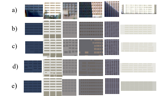
Figure: Comparison with four state-of-the-art methods on a facade parsing. a) Input satellite facades, b) Manually created ground truth. c) The results of applying segmentation to a). d) The results of applying Pix2Pix_96 to a). e) The results of applying DeepFill [30] to a). Our method (e) shows better results than the other methods.
