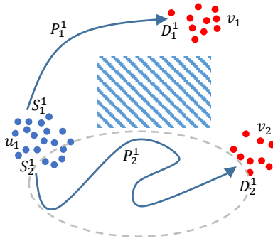
Figure 4: Source and Destination Clustering. Spatial clustering determines clusters u_1 , v_1 , and v_2 which are then used to form the two CMMs \{S_1^1 = u_1', P_1^1, D_1^1 = v_1\} and \{S_2^1 = u_1'', P_2^1, D_2^1 = v_2\} where u_1' is the subset of u_1 that navigates to v_1 and u_1'' = u_1 - u_1' .
