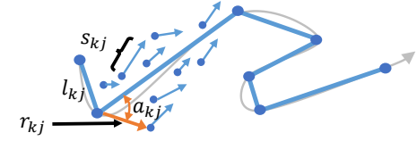
Figure 6: Displacements and Speeds. We associate with each agent a d_{kj} = (r_{kj}, a_{kj}) relative to the closest linear segment start point. We also store with each agent its speed s_{kj} . Blue dots represent agents, line segments are starting points, blue arrows are agents' velocity, and orange arrows represent the angle and the displacement vector respectively.
