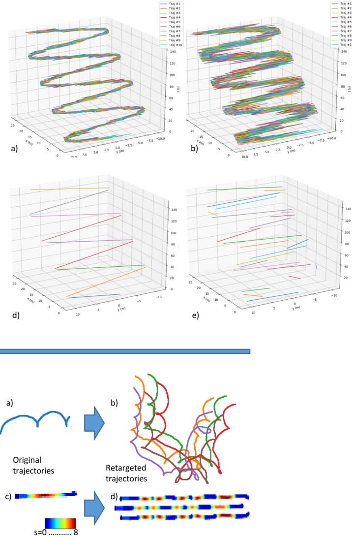
Figure 9: Retarget Examples. a-b) An original trajectory retargetted to multiple agents along a longer U-shaped path. c-d) One stop-n-go agent retargetted to multiple stop-n-go motions by random order retargeting. The color represents speed as per the included JET color map from 0 to 8 m/s.
