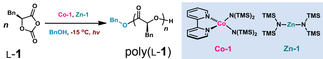
Scheme 3. Photoredox controlled ring-opening polymerization of L-1 mediated by Co-1/Zn-1.
