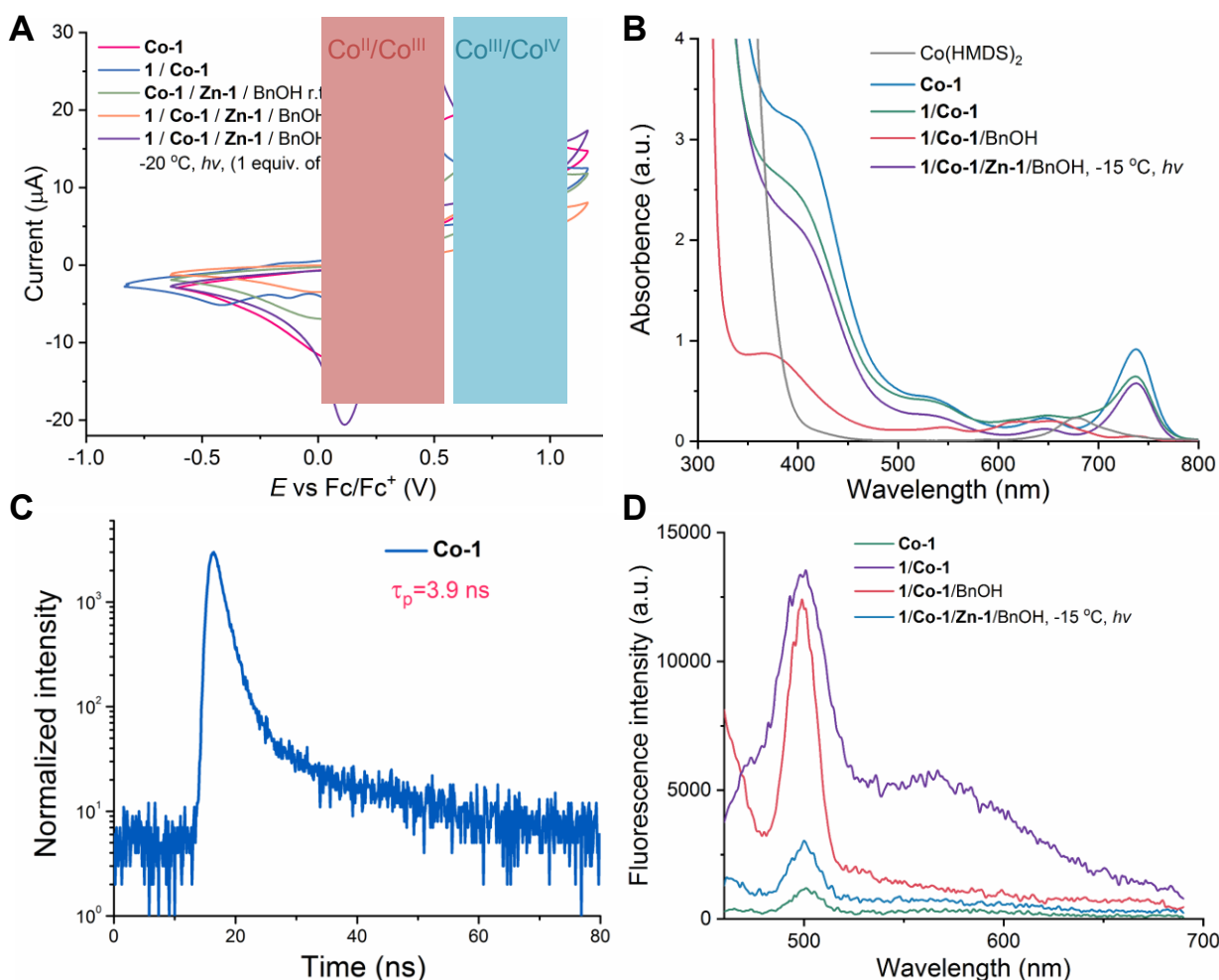
Figure 2. Electrochemical and photophysical studies of the photoredox decarboxylation reactions mediated by Co-1. (A) Cyclic voltammograms of Co-1 and the ring-opening reaction mixtures (1 equiv. of each) at various conditions. Scan rate: 100 mV/s. Solvent: 0.1 M tetrabutylammonium hexafluorophosphate in THF. Initial scanning direction: zero to positive. (B) UV/Vis absorption spectra of Co-1 and the reaction mixtures (1 equiv. of each). [\text{Co}] = 2.0 mM in THF in all samples. (C) Photoluminescence decay of Co-1 recorded in deaerated THF with excitation at 350 nm. (D) Emission spectra of Co-1 and the reaction mixtures (1 equiv. of each) with the excitation at 435 nm. [\text{Co}] = 2.0 mM in THF in all samples.
