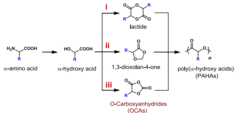
Scheme 1. Synthetic routes of poly( \alpha -hydroxy acids) (PAHAs) from \alpha -amino acids and \alpha -hydroxy acids via different monomers.
