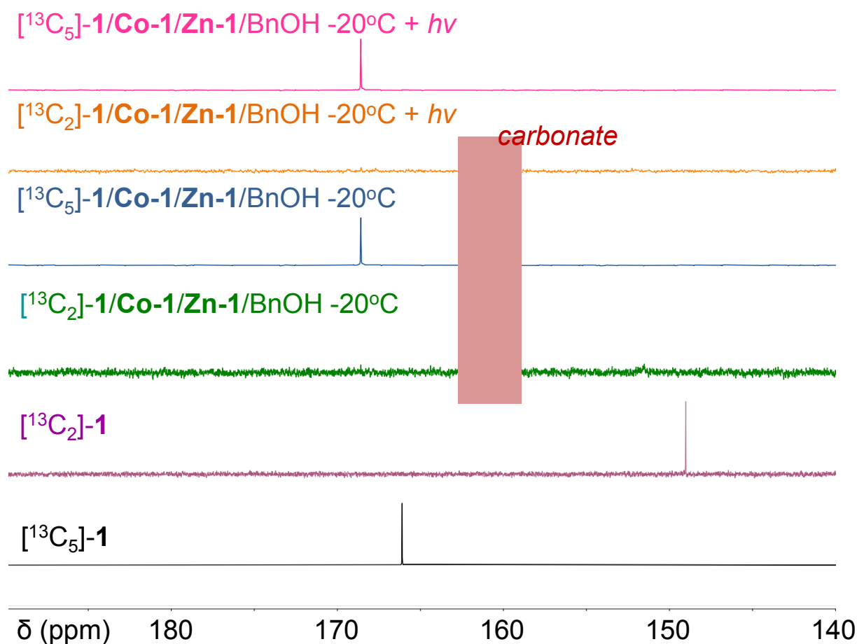
Figure 3. ^{13}\text{C} NMR studies of oxidative addition reactions between L-1 and Co/Zn complexes. To improve the ^{13}\text{C} NMR spectra qualities (due to the paramagnetic Co complexes) and determine the regioselectivity, [^{13}\text{C}_2]\text{-1} and [^{13}\text{C}_5]\text{-1} were used to study the ring-opening reaction (600 MHz, \text{THF-}d_8 ). The red area highlighted in spectra indicates ^{13}\text{C}_2(\text{O}) carbonate peaks. [\text{L-1}]/[\text{Co-1}]/[\text{Zn-1}]/[\text{BnOH}] = 1/1/1/1 .
