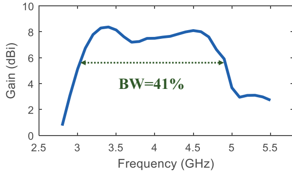
Fig. 5. Peak gain of the wideband U-slot AMC antenna against frequency.
