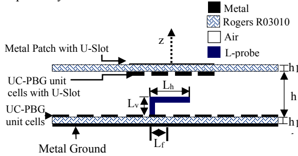
Fig. 1. Side-view of the wideband TE_{10} patch antenna with UC-PBG unit cells in both the patch and the ground plane excited by an L-probe with L_v = 5.535\text{ mm} , L_h = 15\text{ mm} , L_f = 7\text{ mm} , h = 6.4\text{ mm} , and h_1 = 0.635\text{ mm} .
