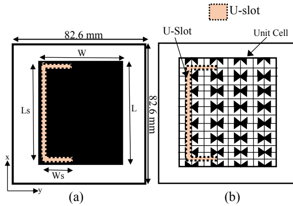
Fig. 2. (a) Top-view of the patch with PEC metal plate with a U-slot (b) Bottom-view of the patch with unit cells and U-slot placed exactly below the PEC metal plate with dimensions of L \times W = 46.2\text{mm} \times 26.4\text{mm} ; L_s = 46\text{mm} , W_s = 6\text{mm} .
