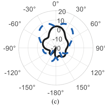
Fig. 6. Radiation patterns of the wideband AMC U-slot patch antenna at (a) 3.2 GHz, (b) 3.9 GHz and (c) 4.6 GHz; E-plane: solid black line, H-plane: dashed blue line.
