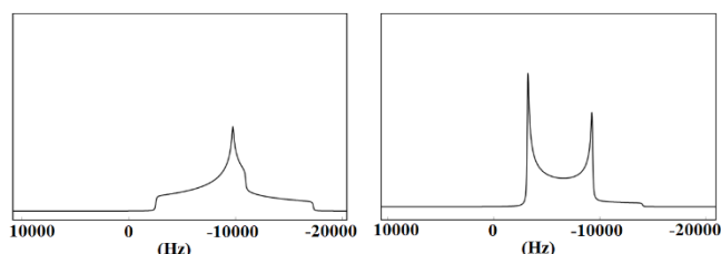
Figure 4. Representative spectral simulation (using DMFit) for ^{23}\text{Na} (Spin = 3/2 ) with a quadrupolar coupling constant ( C_Q ) of 4.5 MHz and quadrupolar asymmetry parameters, \eta of 1 (left) and 0 (right) under static conditions. These patterns represent the central transitions of spin 3/2 ( ^{23}\text{Na} ), broadened by quadrupolar interaction to the second order, under magic angle spinning (MAS).
