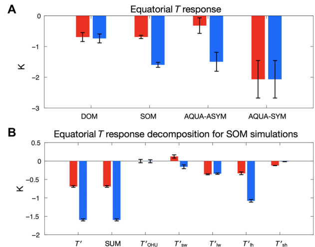
Fig. 5. Equatorial surface temperature response. (A) The surface temperature response averaged over 5°S to 5°N and all longitudes. (B) The attribution of equatorial surface temperature response in the SOM experiments (see Materials and Methods). The NH forcing case is shown in red, and the SH forcing case is shown in blue. Black error bars indicate the 95% confidence level based on a two-sided t test.
