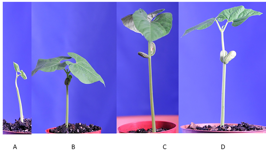
FIG. 11: Seedlings after 7-day growth: (A) untreated and (B) 0.5-min, (C) 1-min, and (D) 15-min CPJ
