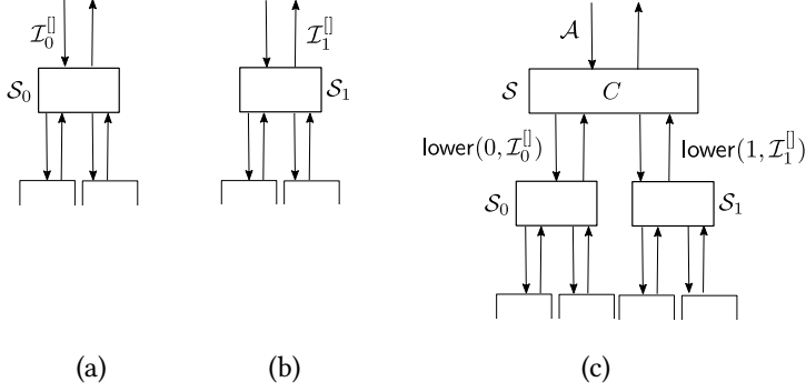
Fig. 5. Illustration of Lowering. (a) Stack S_0 and its specification T_0^[] . (b) Stack S_1 and its specification T_1^[] . (c) Stack S that composes S_0 and S_1 as subcomponents. To prove the assertion A for S , it is sound to assume the lowering of T_0^[] and T_1^[] , and derive A in TLC, i.e., \text{lower}(i, T_i^[]) \vdash_c A .
