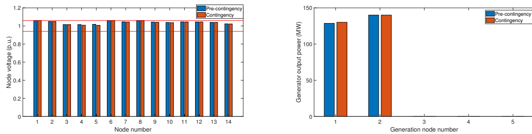
Figure 5. Voltage and power dispatched implementing the QCQP results in a power flow of the network prior to and after contingency of branch 5 (generation nodes are, respectively, 1, 2, 3, 6, and 8).
