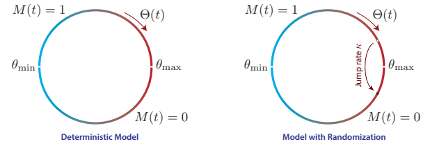
Fig. 1: State space for a water heater under hysteresis control: left hand side shows behavior with deterministic hysteresis control, and right hand side shows behavior under local randomized control
