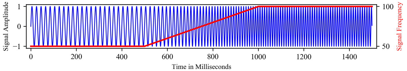
FIGURE 7. PHASE COHERENT FREQUENCY SWEEP FOR EVALUATION
