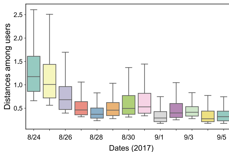
Fig. 9 The latent distances among active users each day. This box plot shows four quartiles of the distribution of the latent distances. The average latent distance is the middle line in each box and the upper and lower boundaries of the box show the third and first quartile of the latent distance in each day. The unit of the latent distance is 1, so the y-axis is the absolute value of the latent distances among users
